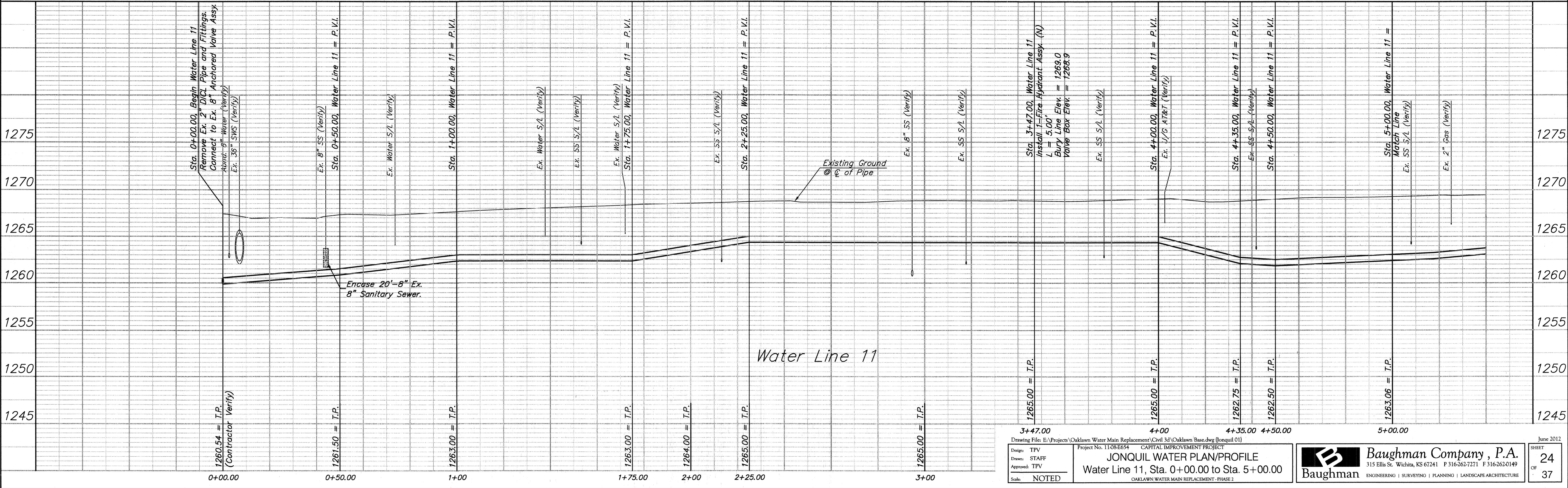
Water Line 11
