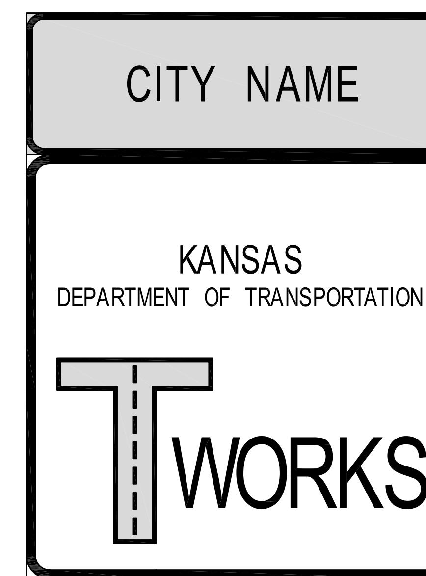
TYPICAL SIGN ASSEMBLY
