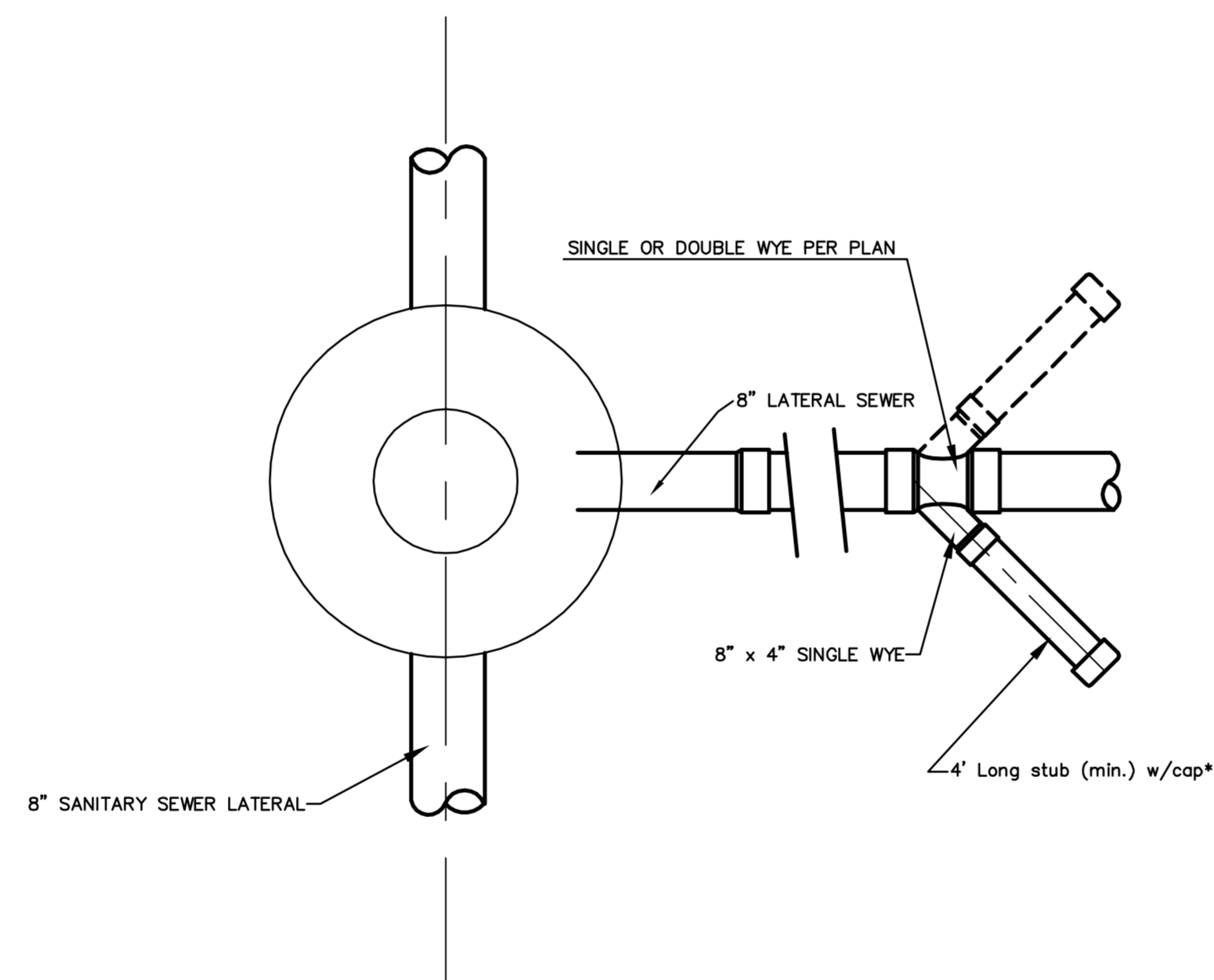
CLEANOUT RISER ASSEMBLY DETAIL W/ MANHOLE CONNECTION
