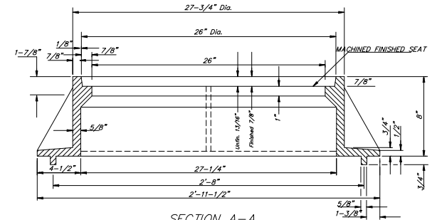
SECTION A-A STANDARD MANHOLE FRAME Weight = 250 Lbs.
