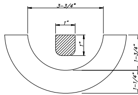
SECTION VIEW
