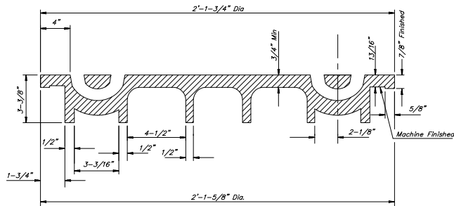
SECTION VIEW
