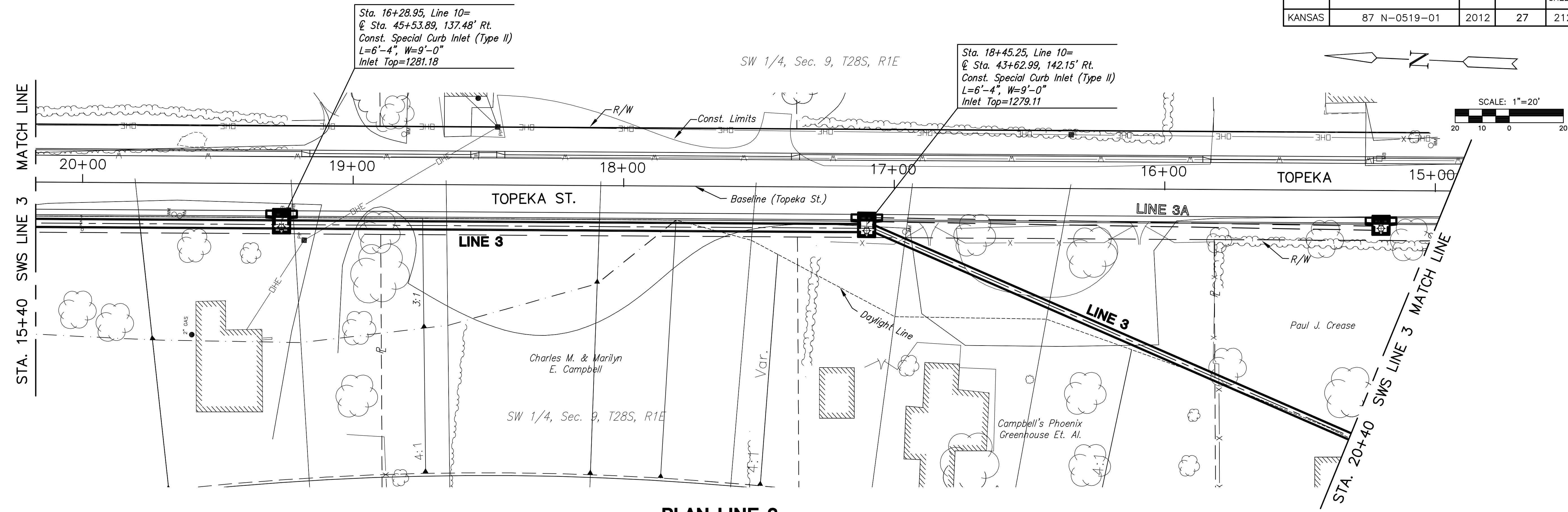
PLAN LINE 3
