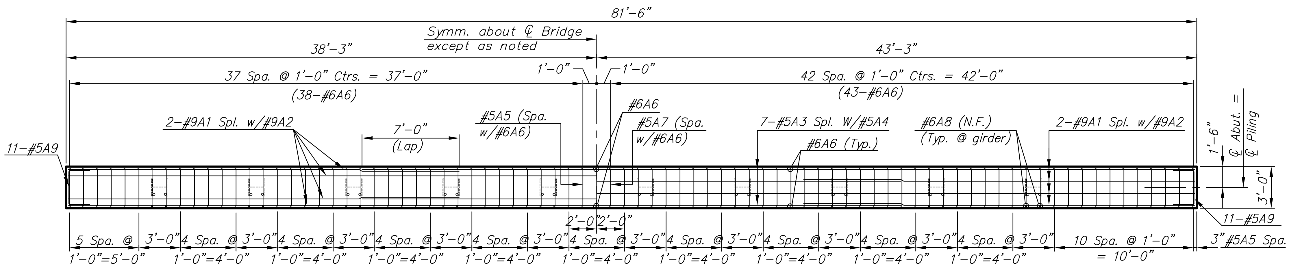
(Reinforcing Steel in Bottom of Abutment Beam)
