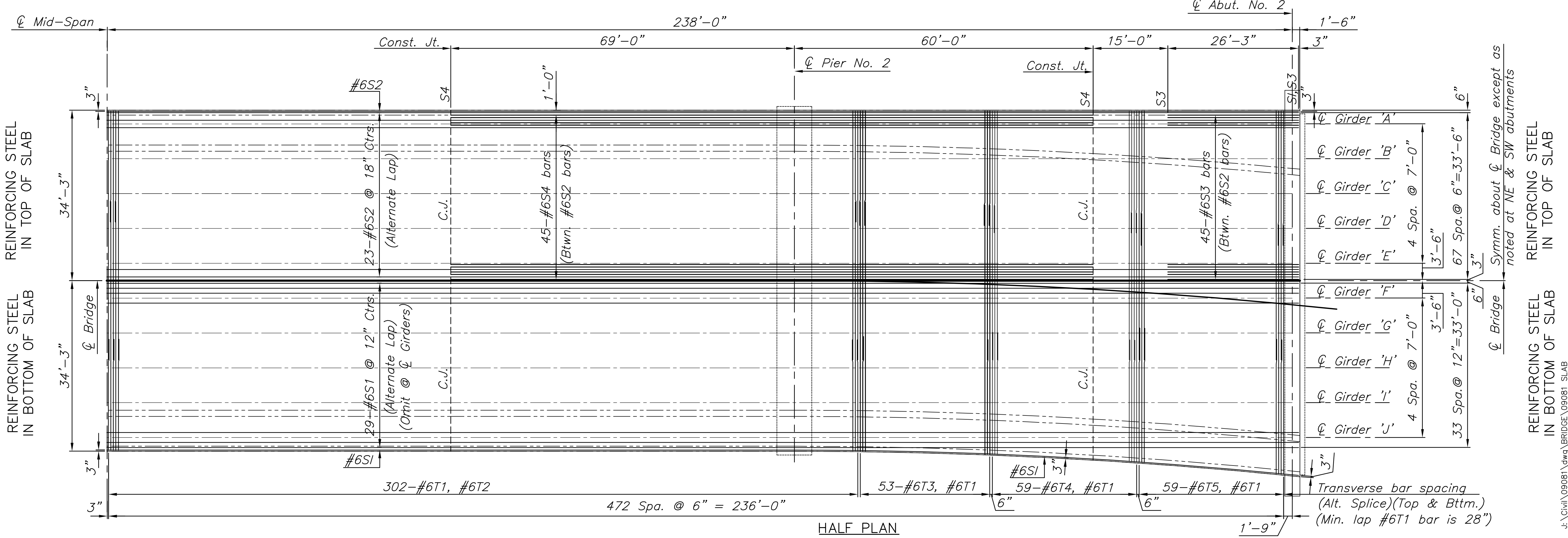
HALF PLAN
