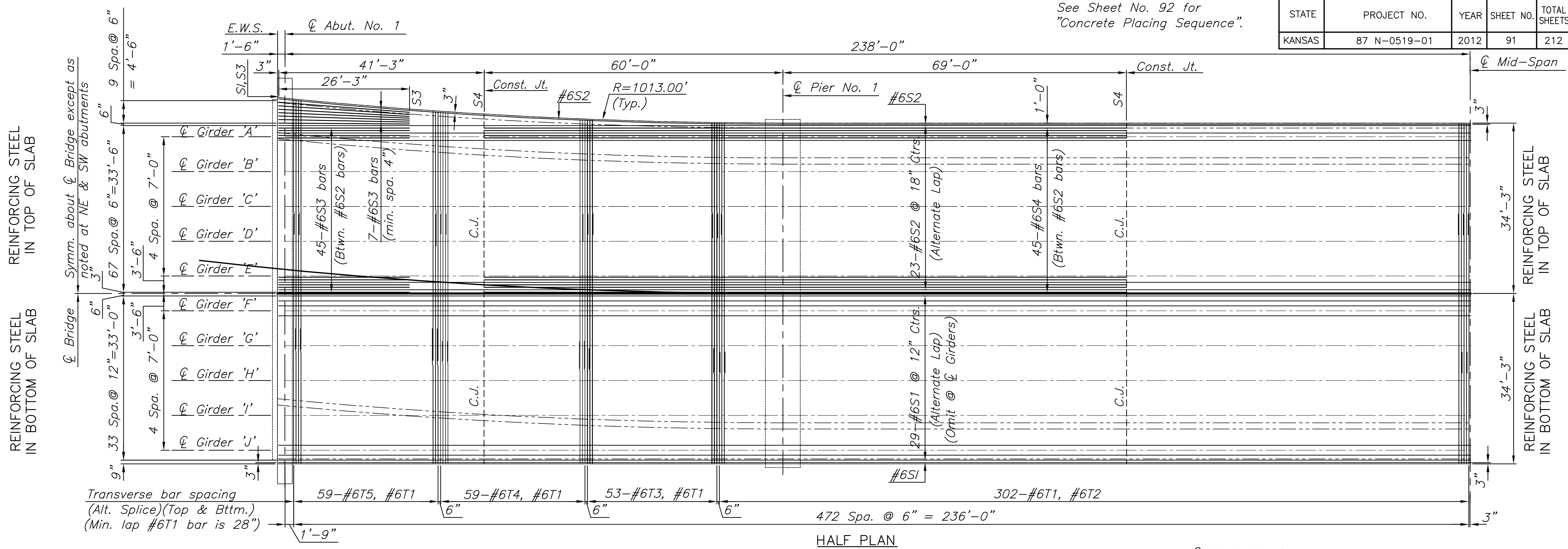
HALF PLAN
