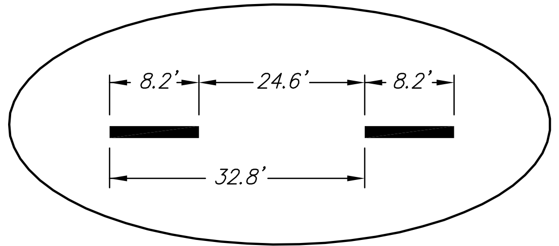
TYPICAL SPACING FOR 6" BROKEN WHITE LANE LINES
