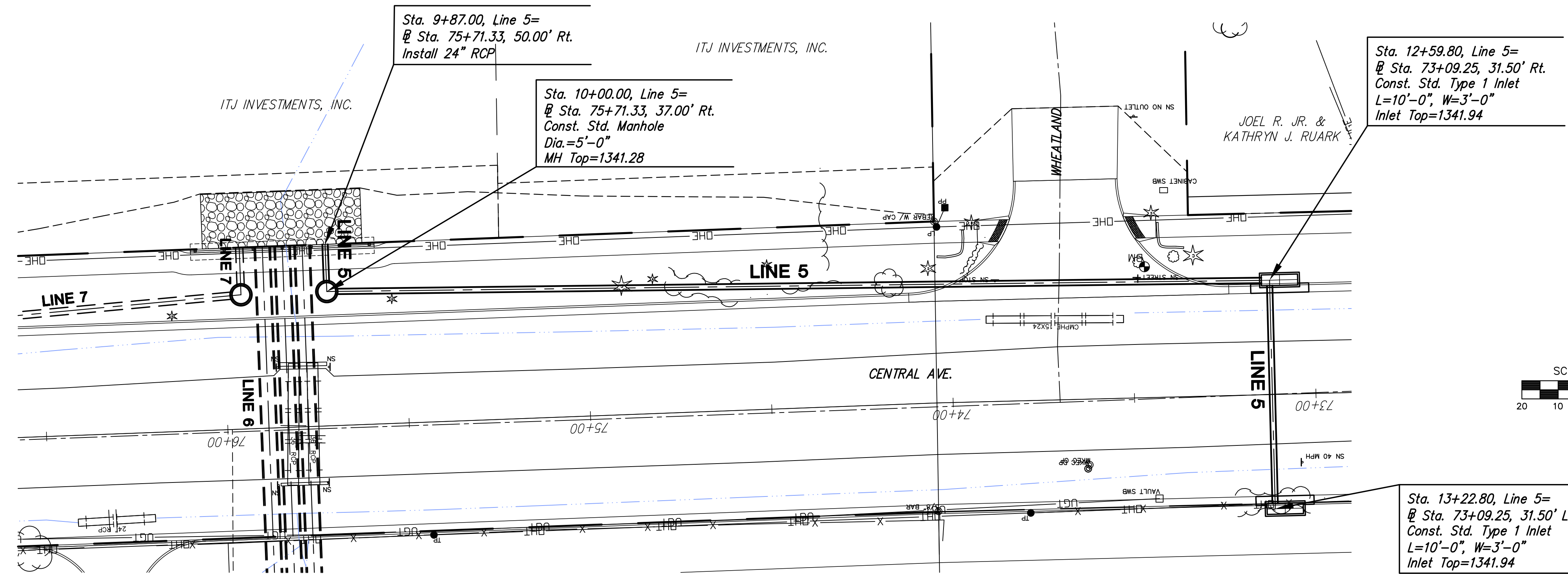
PLAN LINE 5
