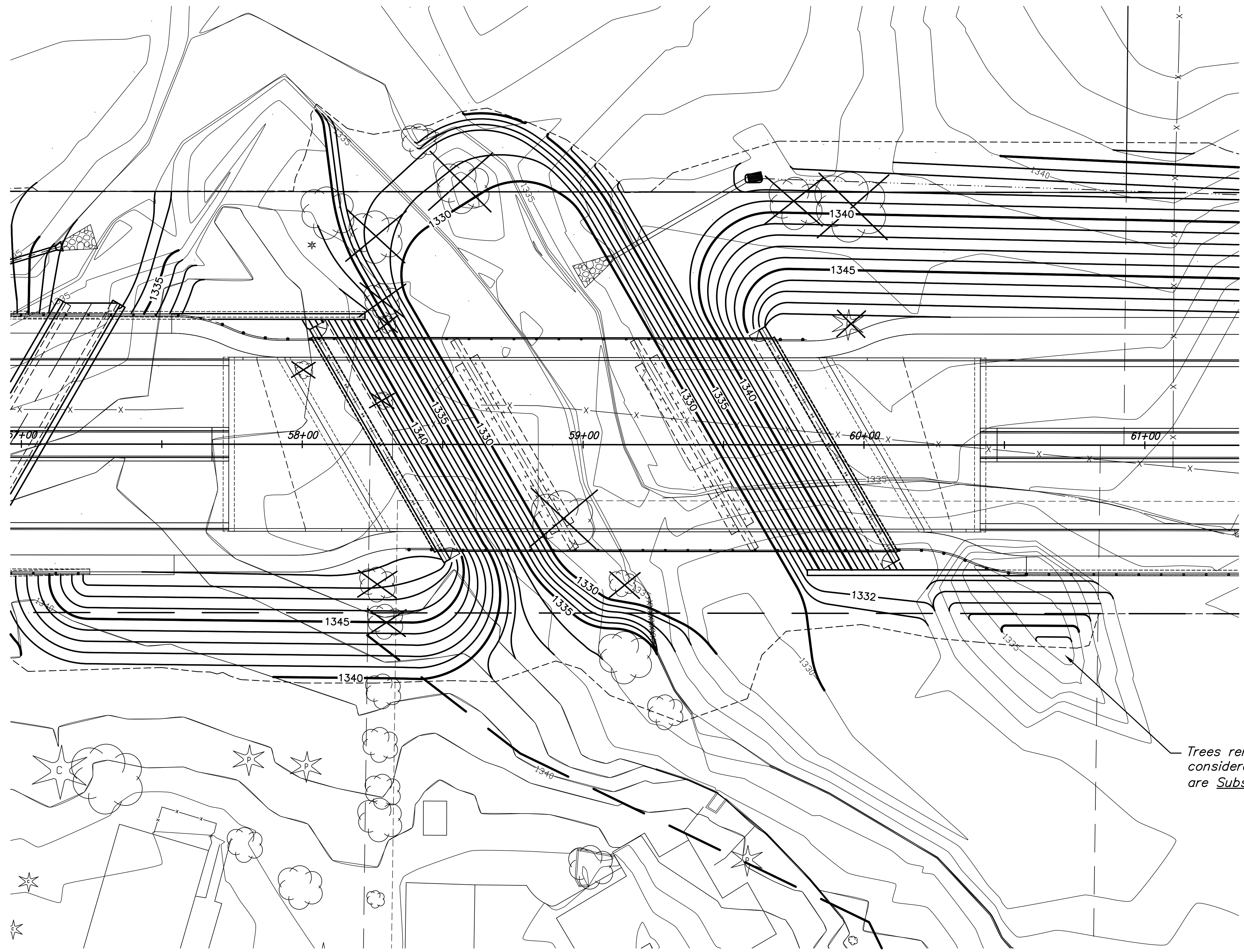
SITE GRADING AND RESTORATION
