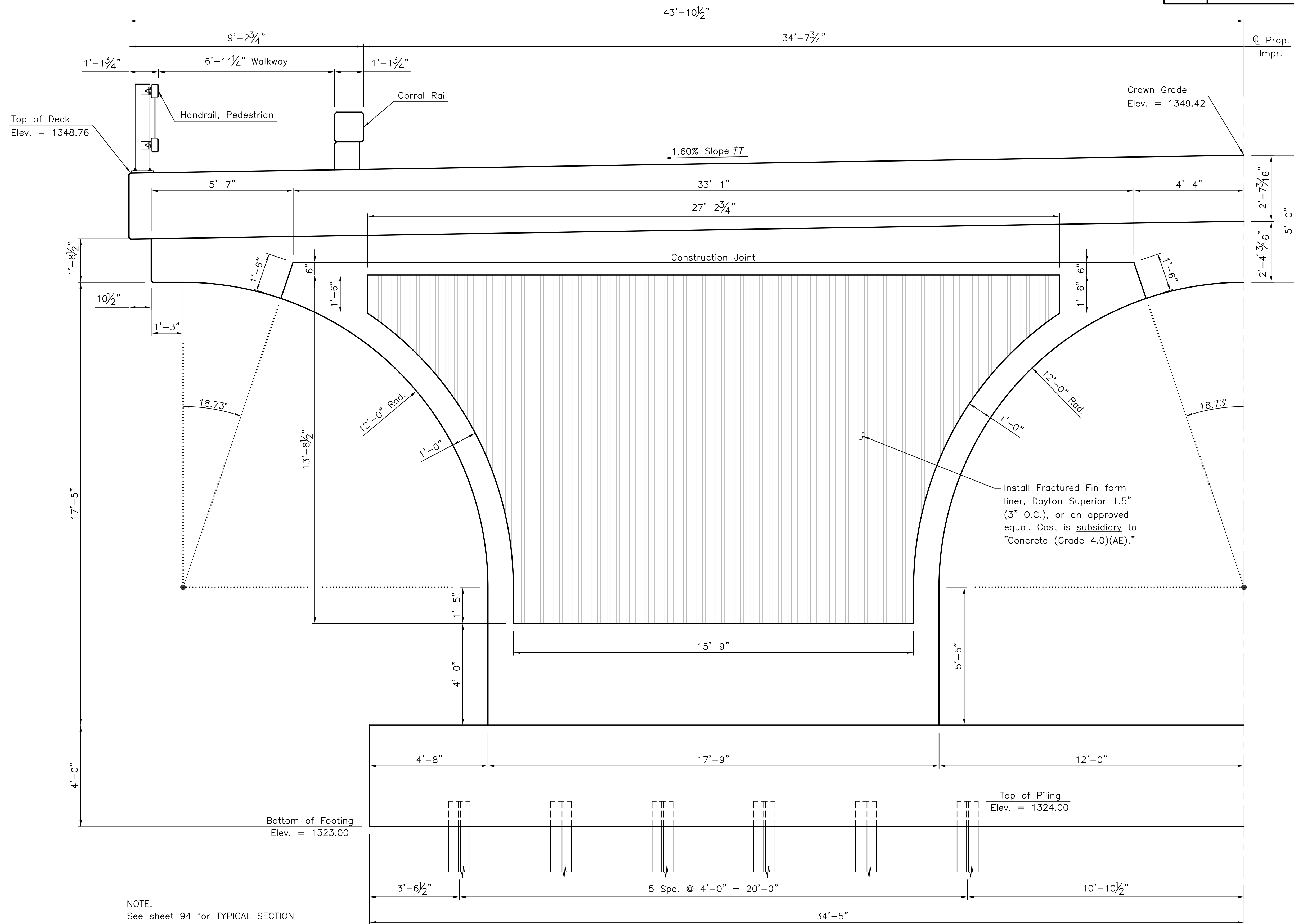
HALF ELEVATION (Measured Along \phi Pier) (Looking Up Station, Pier No. 2) (Looking Down Station, Pier No. 1) †† Cross slope perpendicular to \phi Prop. Impr.
