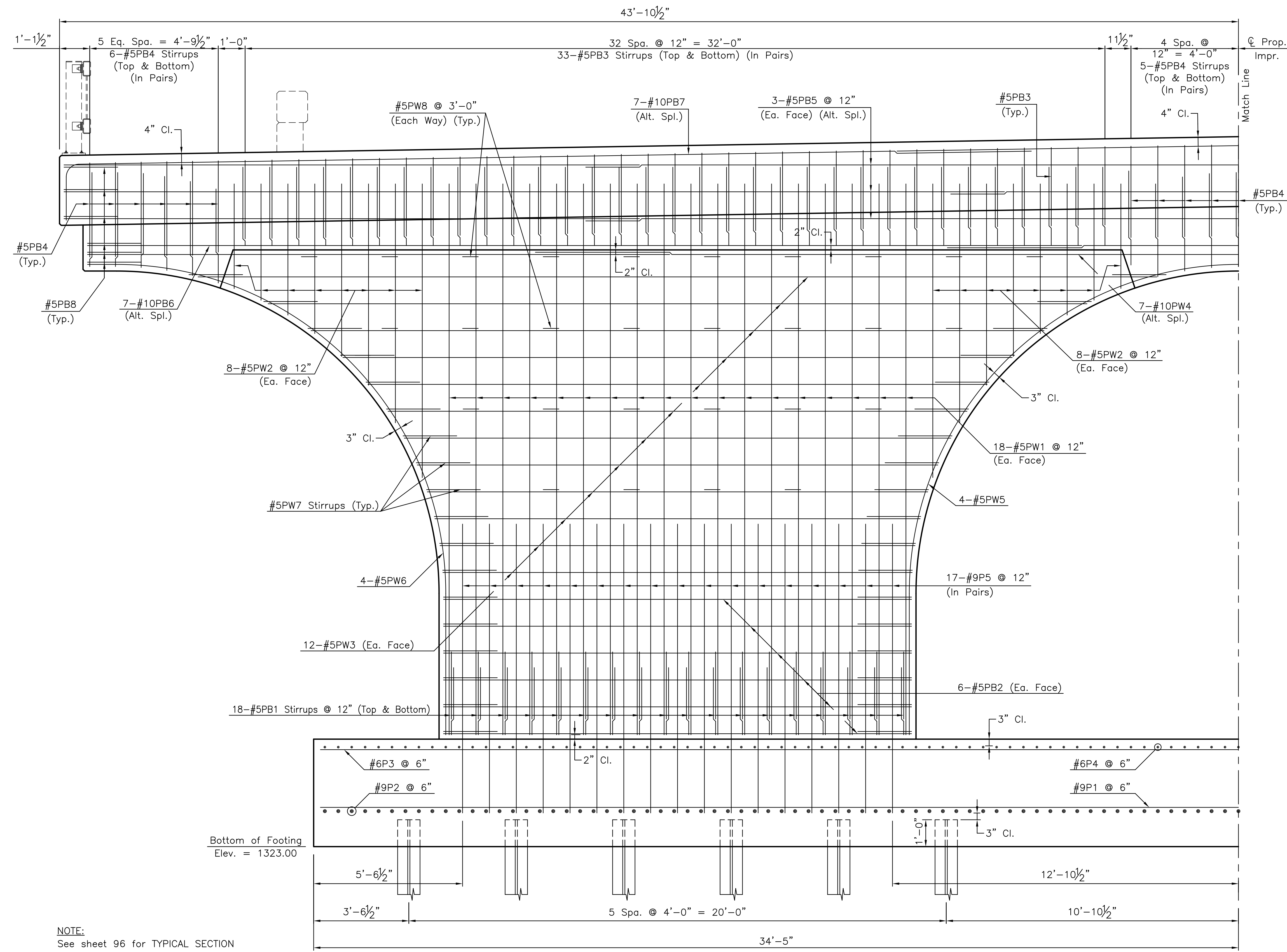
HALF ELEVATION (Measured Along \text{\textcircled{C}} Pier) (Looking Up Station, Pier No. 2) (Looking Down Station, Pier No. 1) †† Cross slope perpendicular to \text{\textcircled{C}} Prop. Impr.
