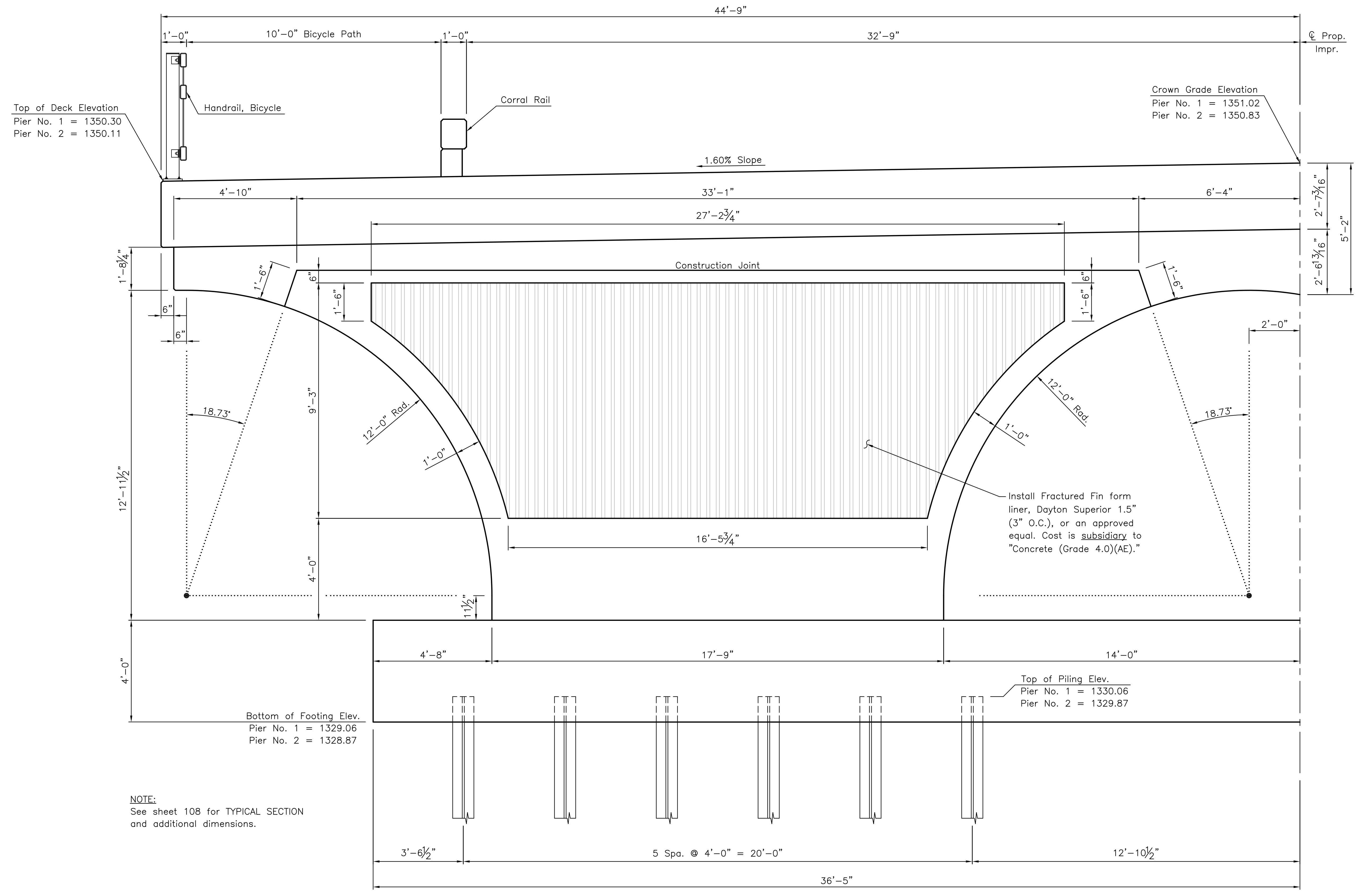
HALF ELEVATION (Looking Up Station)
