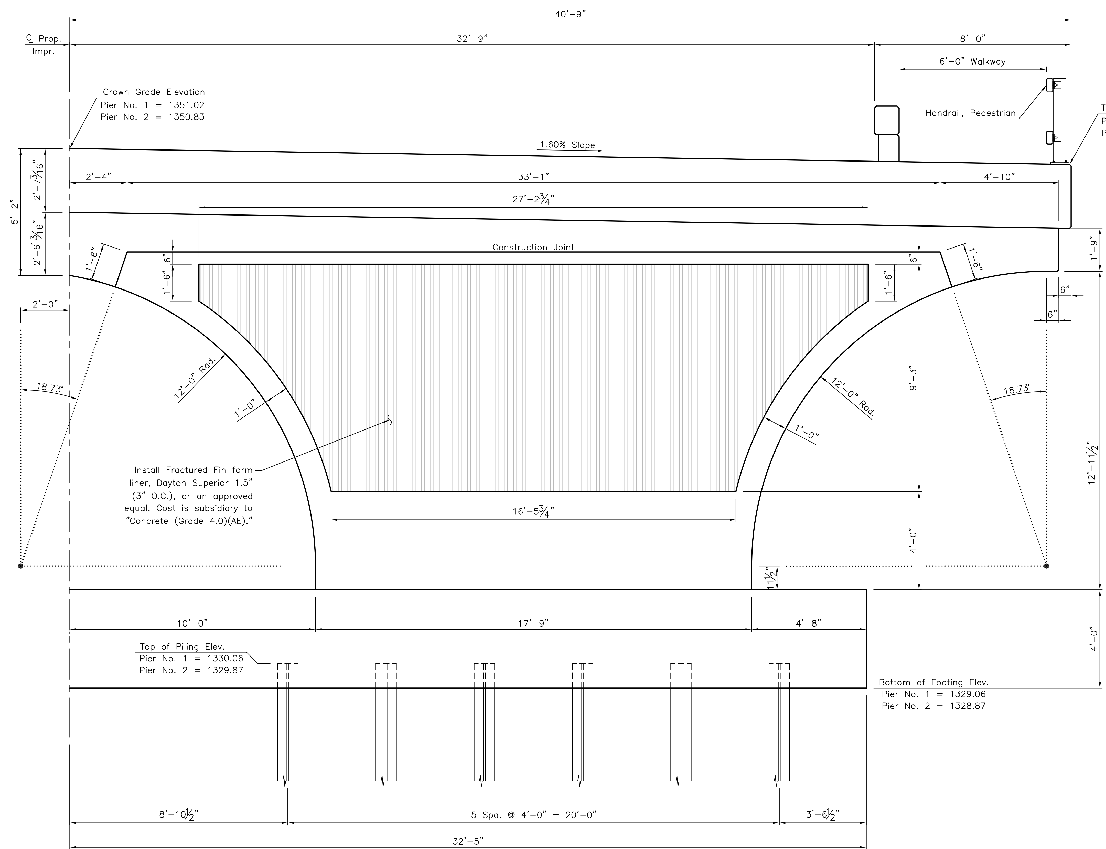
HALF ELEVATION (Looking Up Station)
