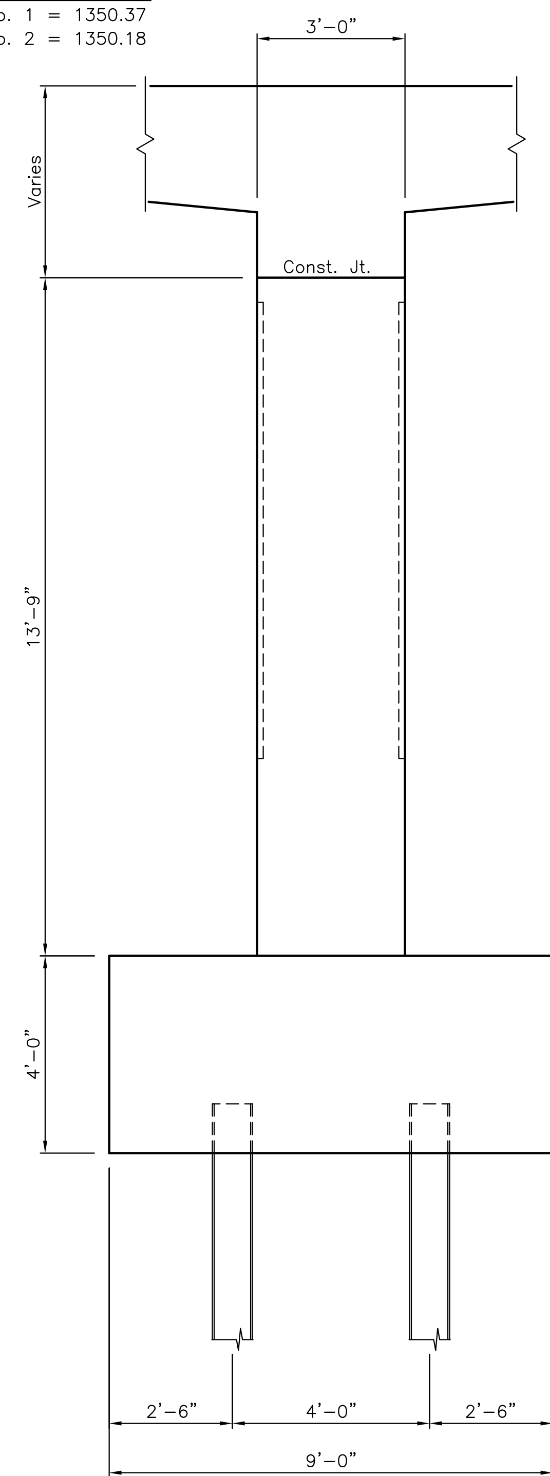
TYPICAL SECTION
