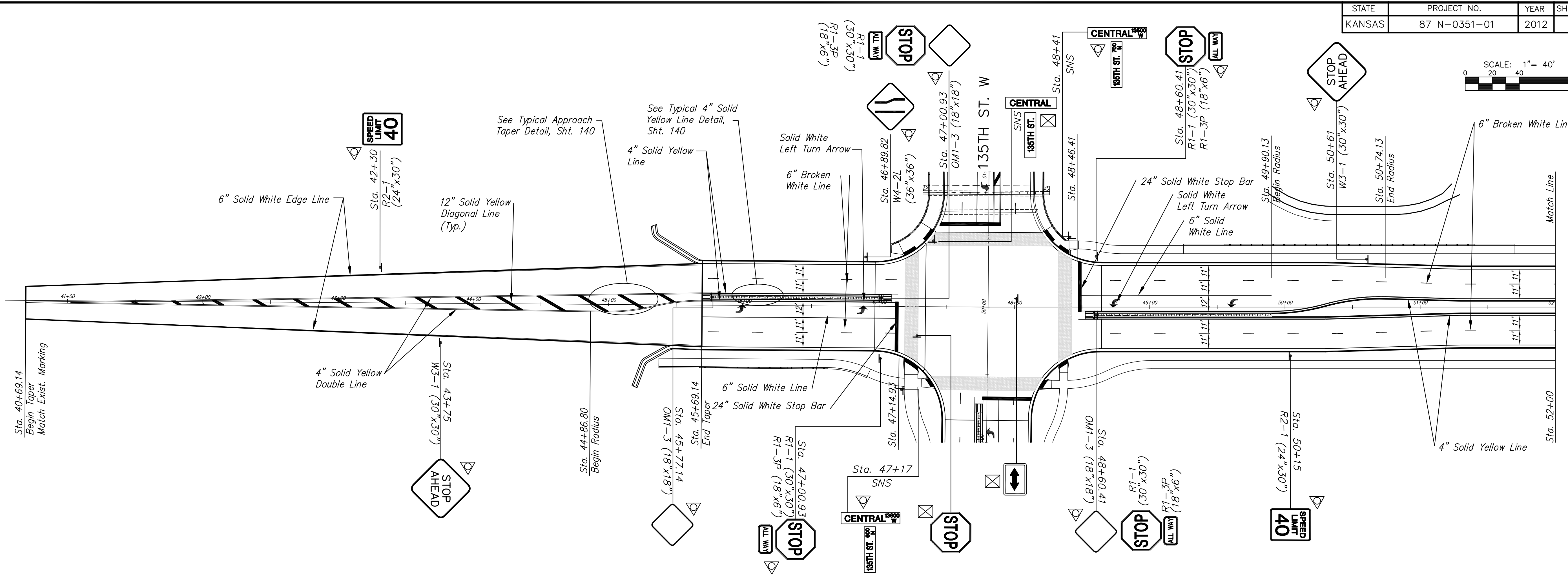
PLAN - CENTRAL AVE.
