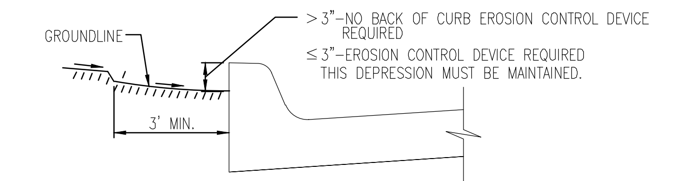
CURB BACKFILL DETAIL THIS IS A TEMPORARY MEASURE ONLY, WHEN APPROVED BY THE PROJECT ENGINEER. THE DIRT GRADE BEHIND THE CURB SHALL BE BROUGHT TO THE TOP OF CURB, WITH TEMPORARY EROSION CONTROL MAT OR PERMANENT VEGETATION PLACED, PRIOR TO THE COMPLETION OF ALL PROJECTS.
