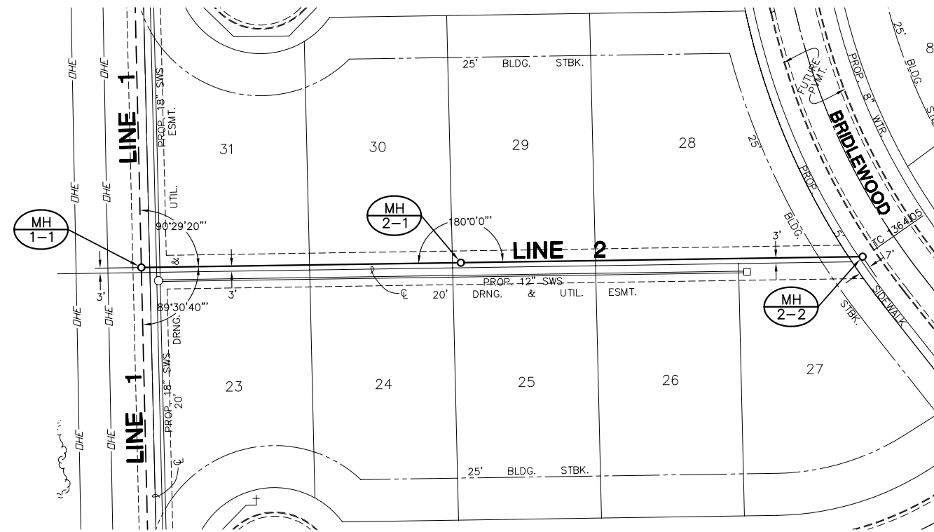
PLAN LINE 2
