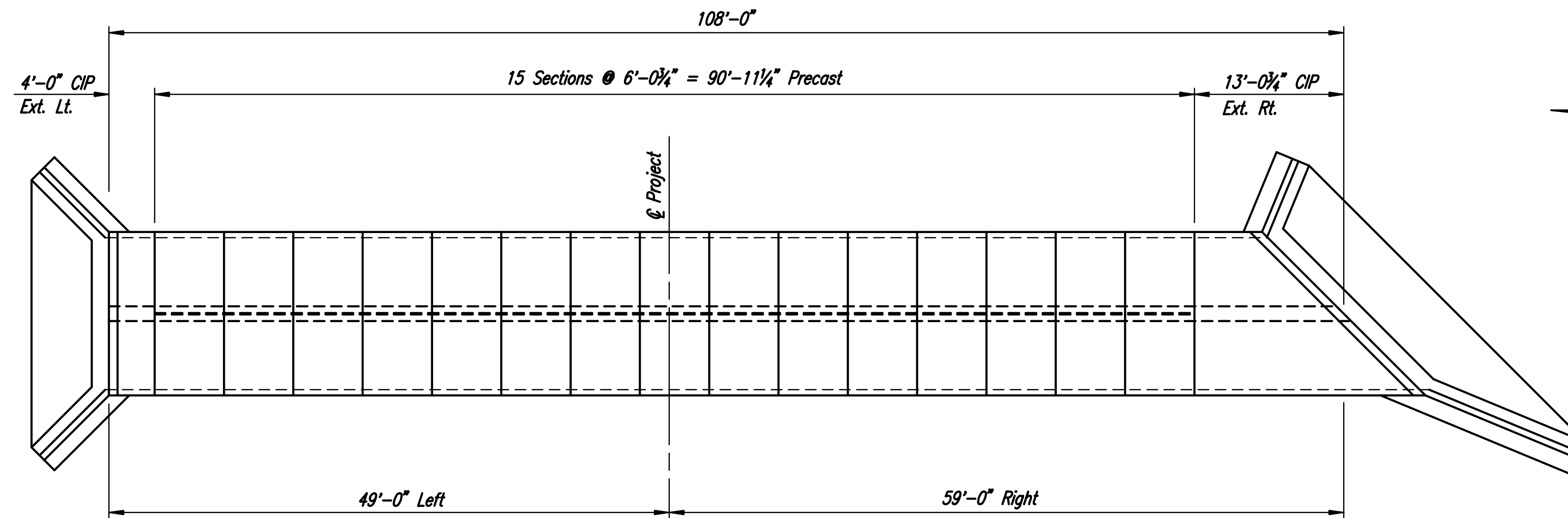
PLAN
