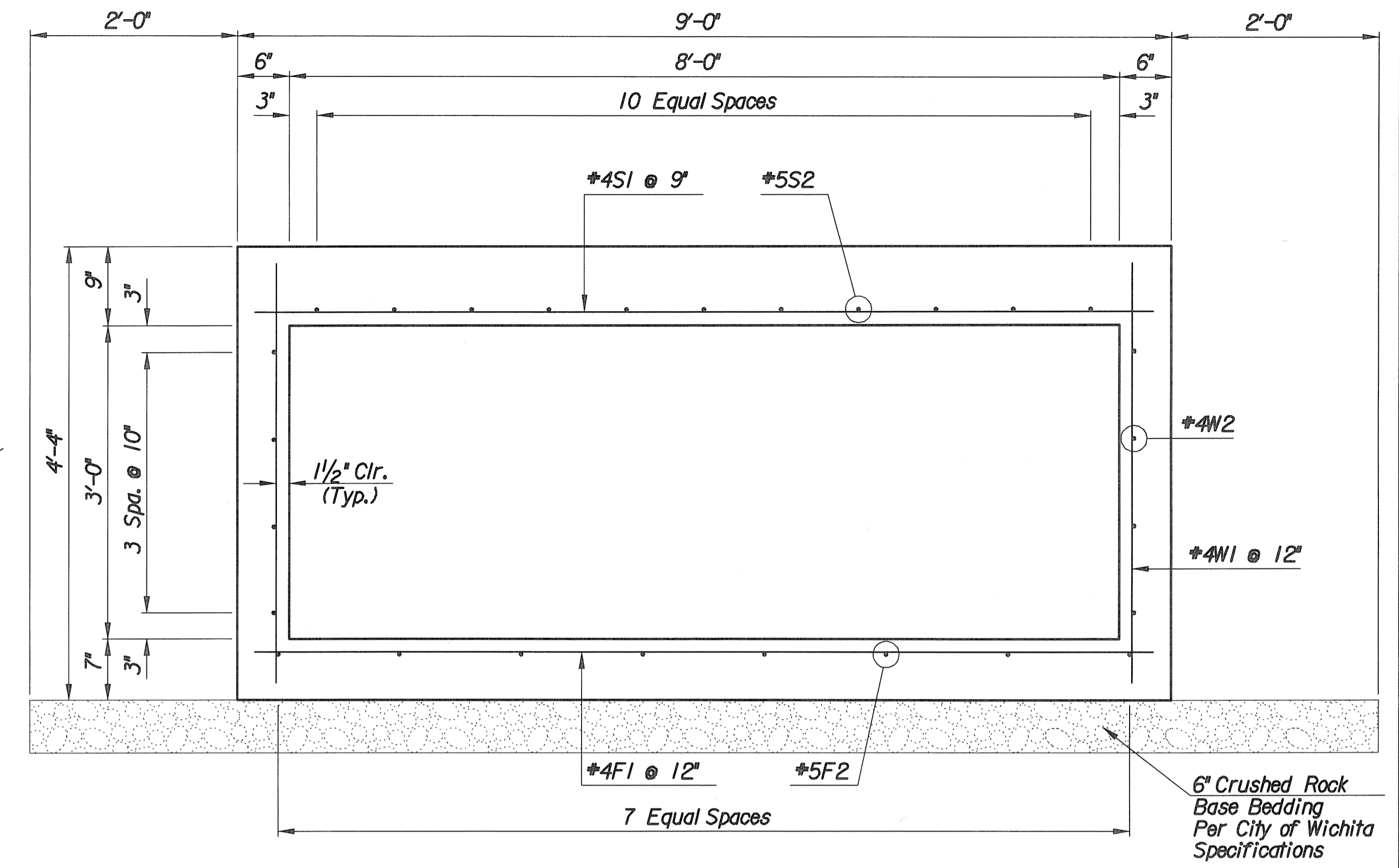
SECTION
