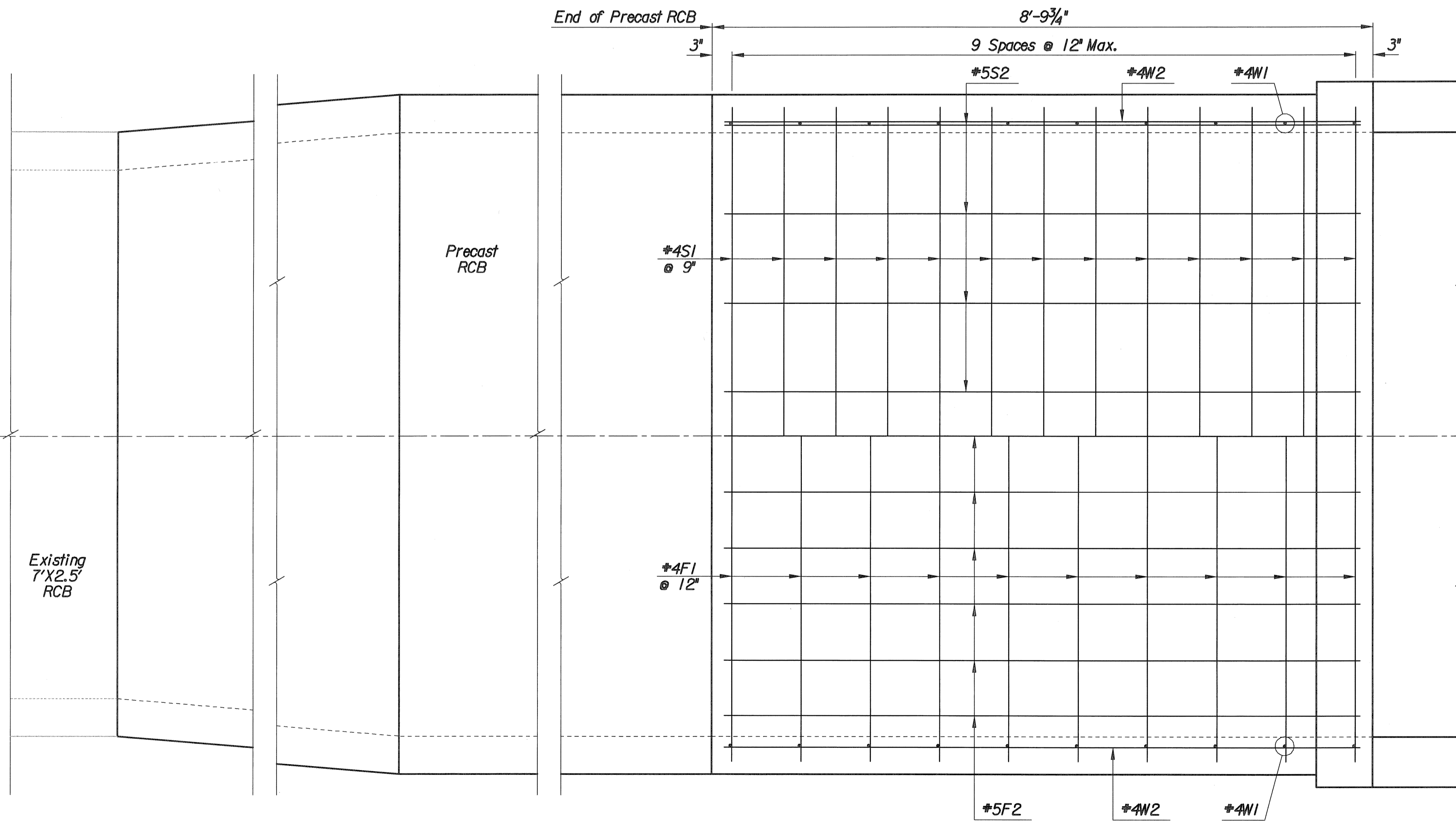
PLAN
