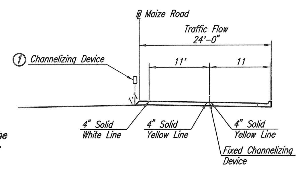
STAGE I TYPICAL TRAFFIC CONTROL SPACING
