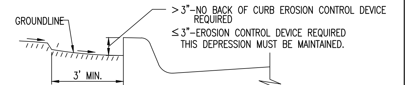
CURB BACKFILL DETAIL
