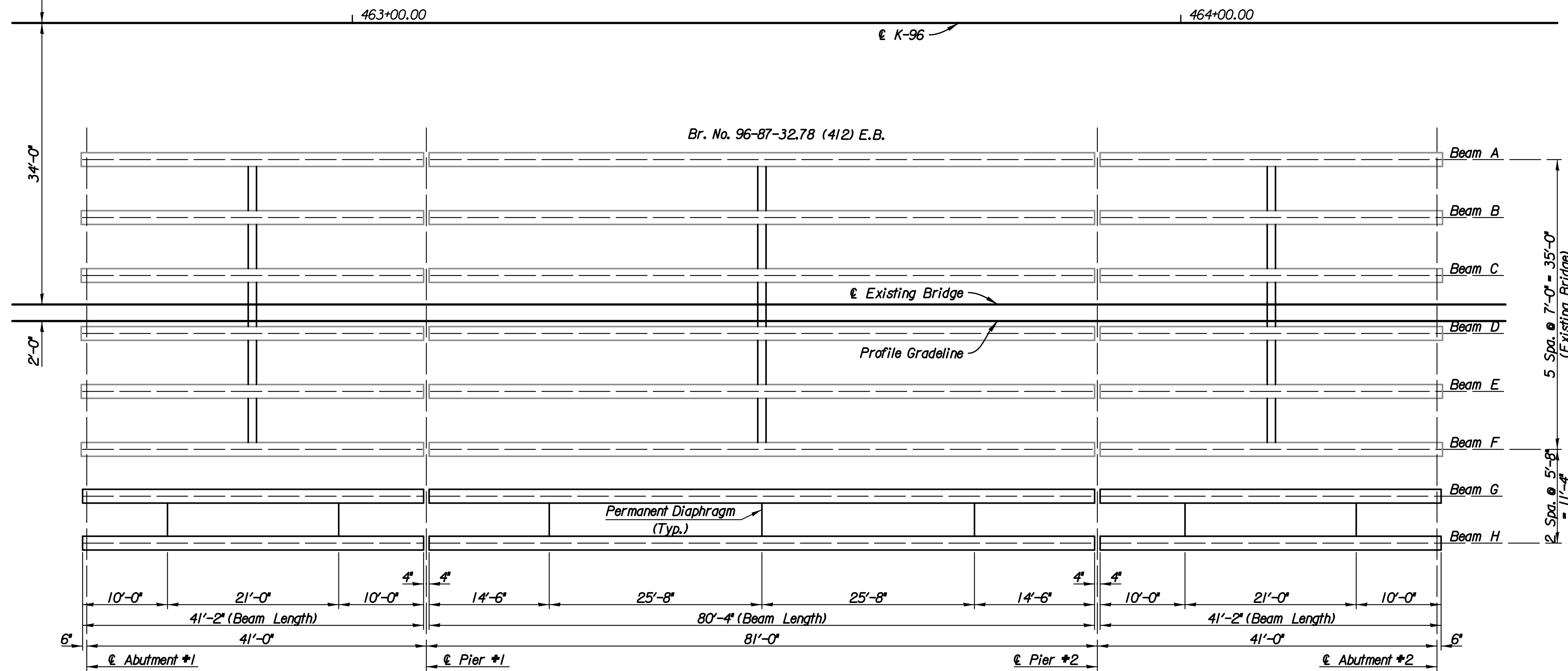
FRAMING PLAN
