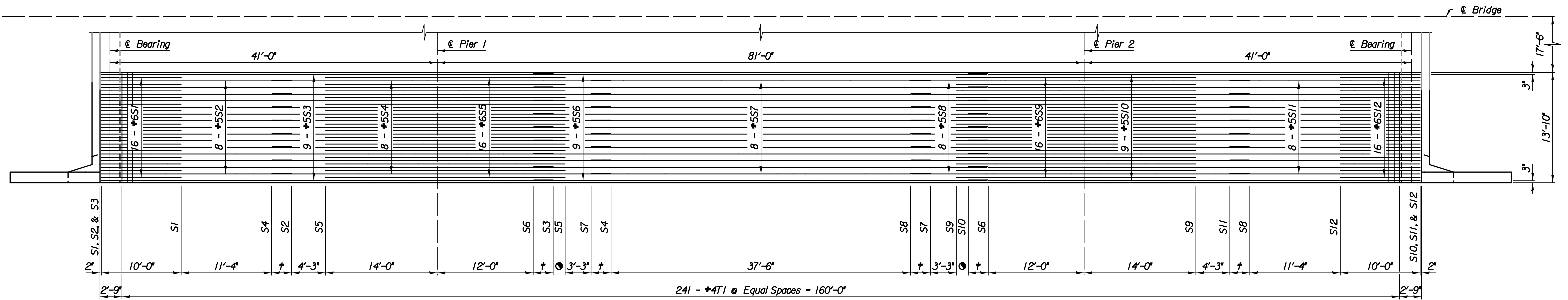
TOP SLAB PLAN (WIDENING)
