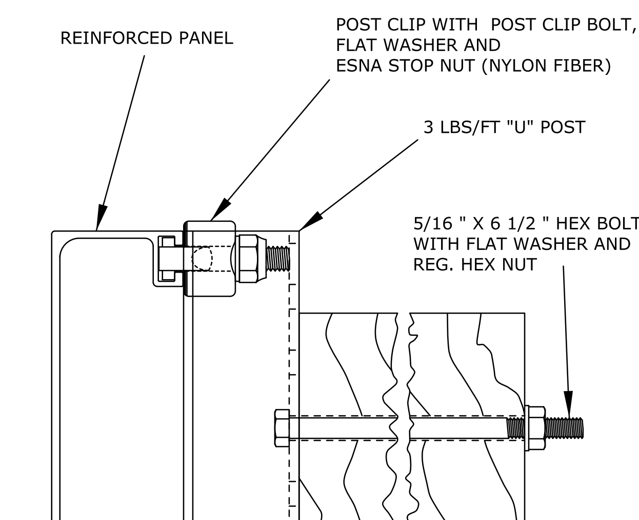
SIDE VIEW
