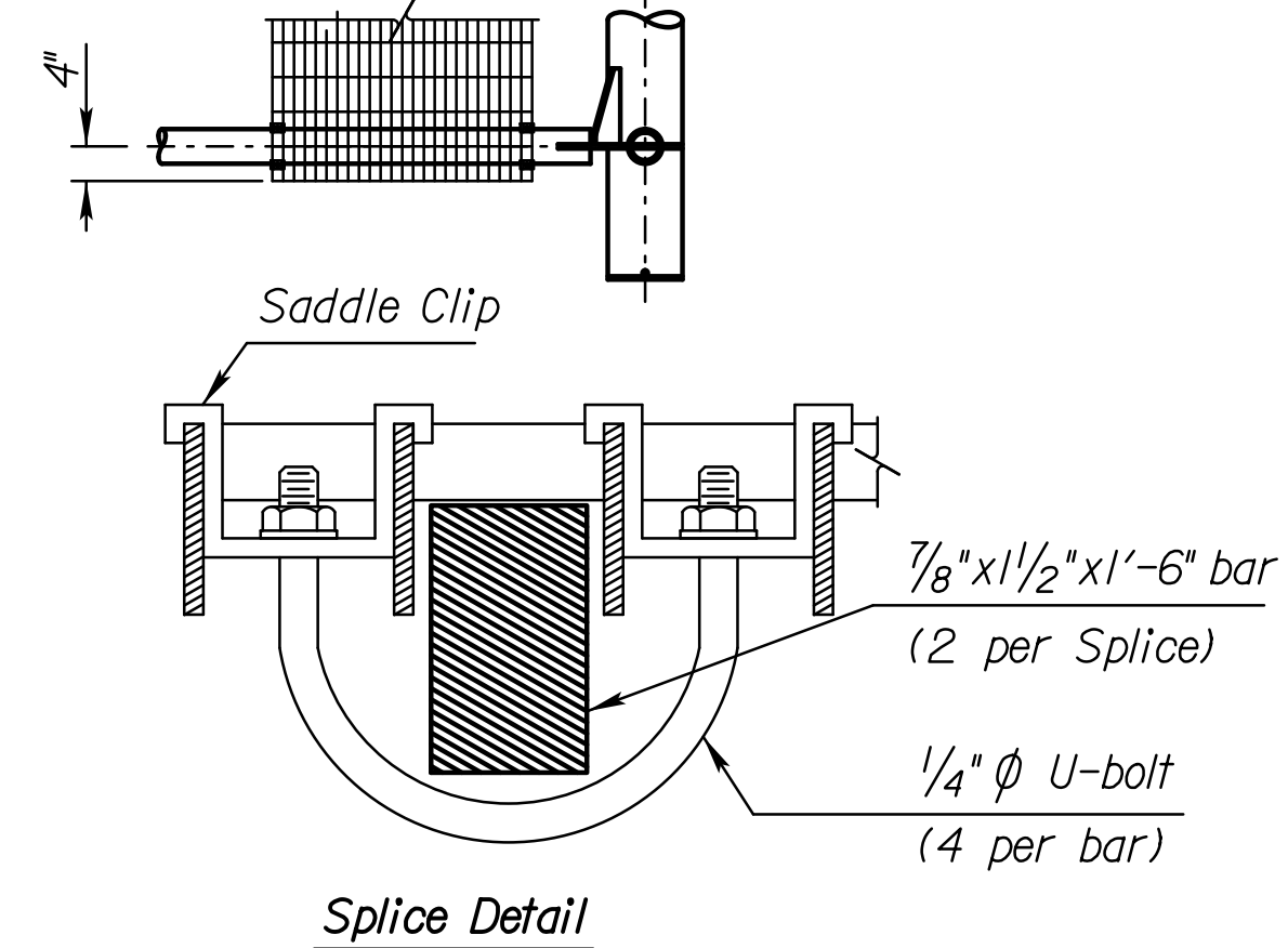
INTERIOR GRATE CONNECTION DETAILS
