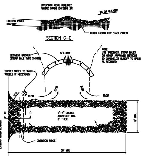
STABILIZED CONSTRUCTION ENTRANCE
