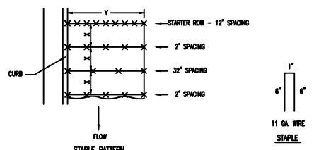
DETAILS FOR APPROVED EROSION CONTROL MAT
