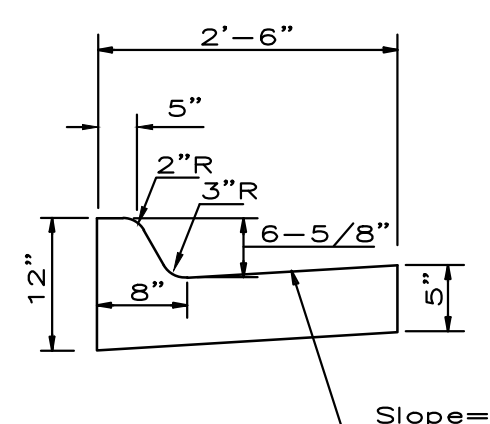
COMBINED CURB & GUTTER
