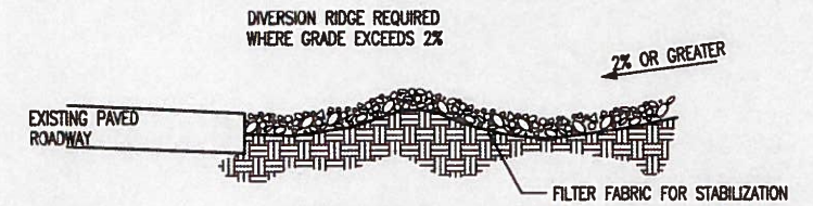
SECTION C-C
