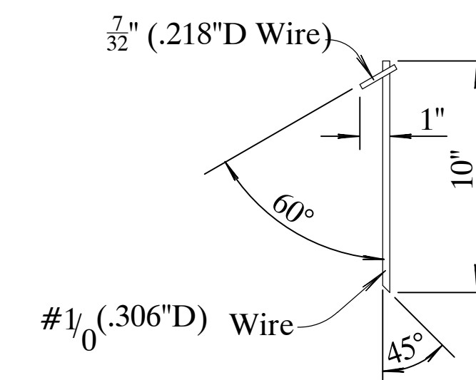
STAKE DETAIL (6 Pieces minimum required)
