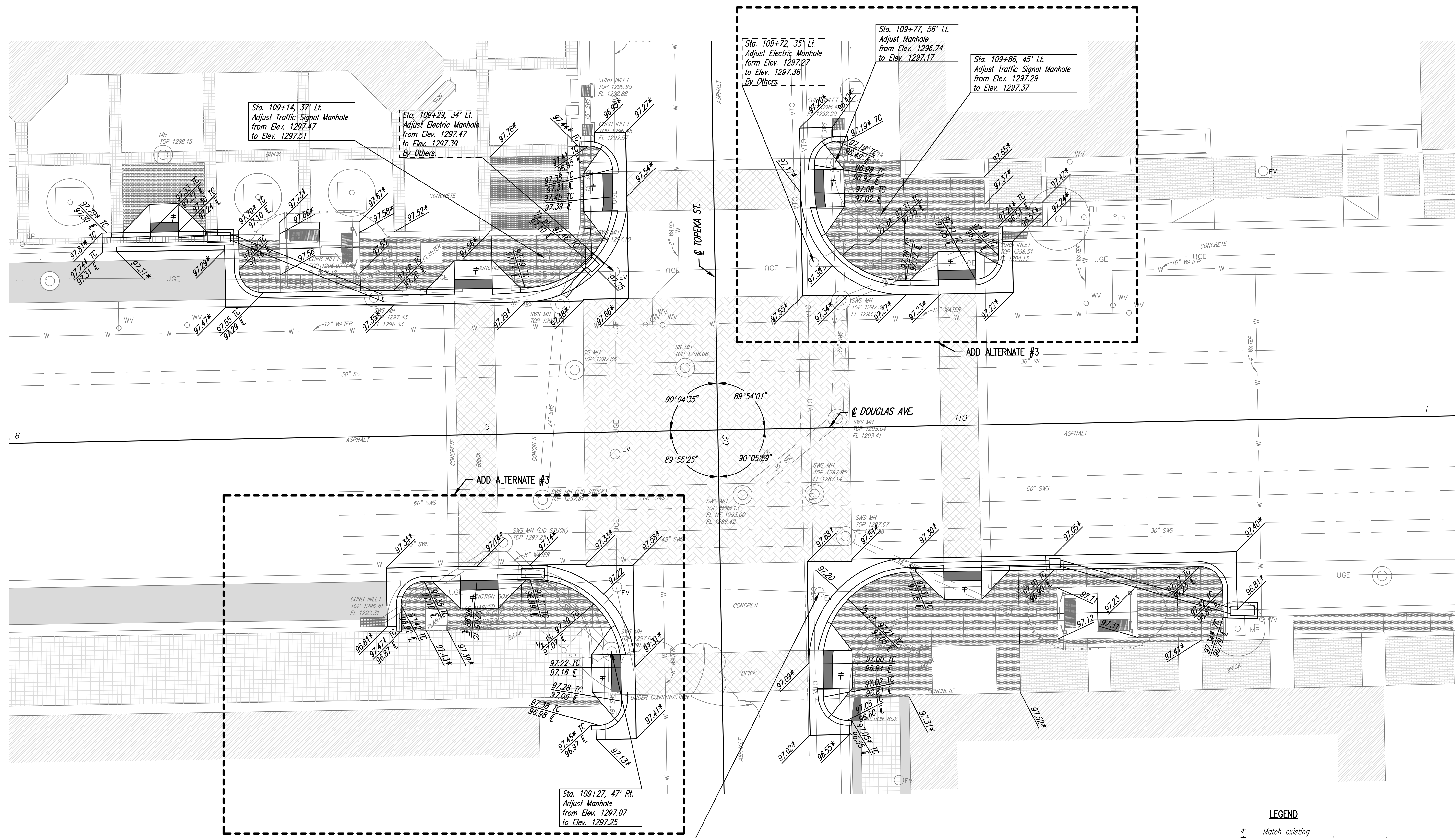
CIVIL PLAN 1"=10'-0" NORTH
