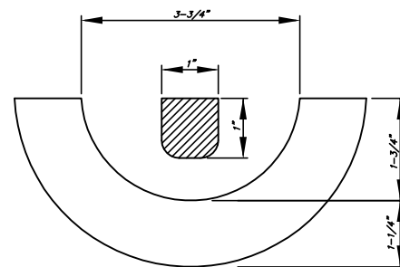
SECTION VIEW
