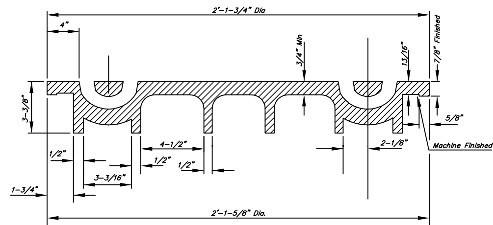
SECTION VIEW
