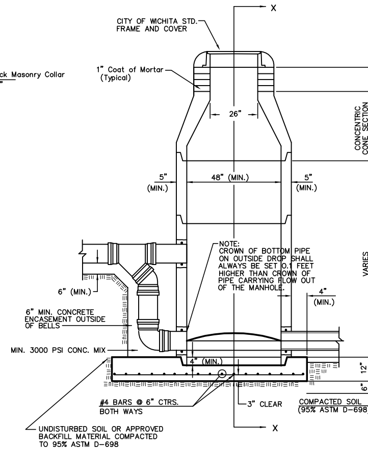
TYPE P OUTSIDE DROP MANHOLE
