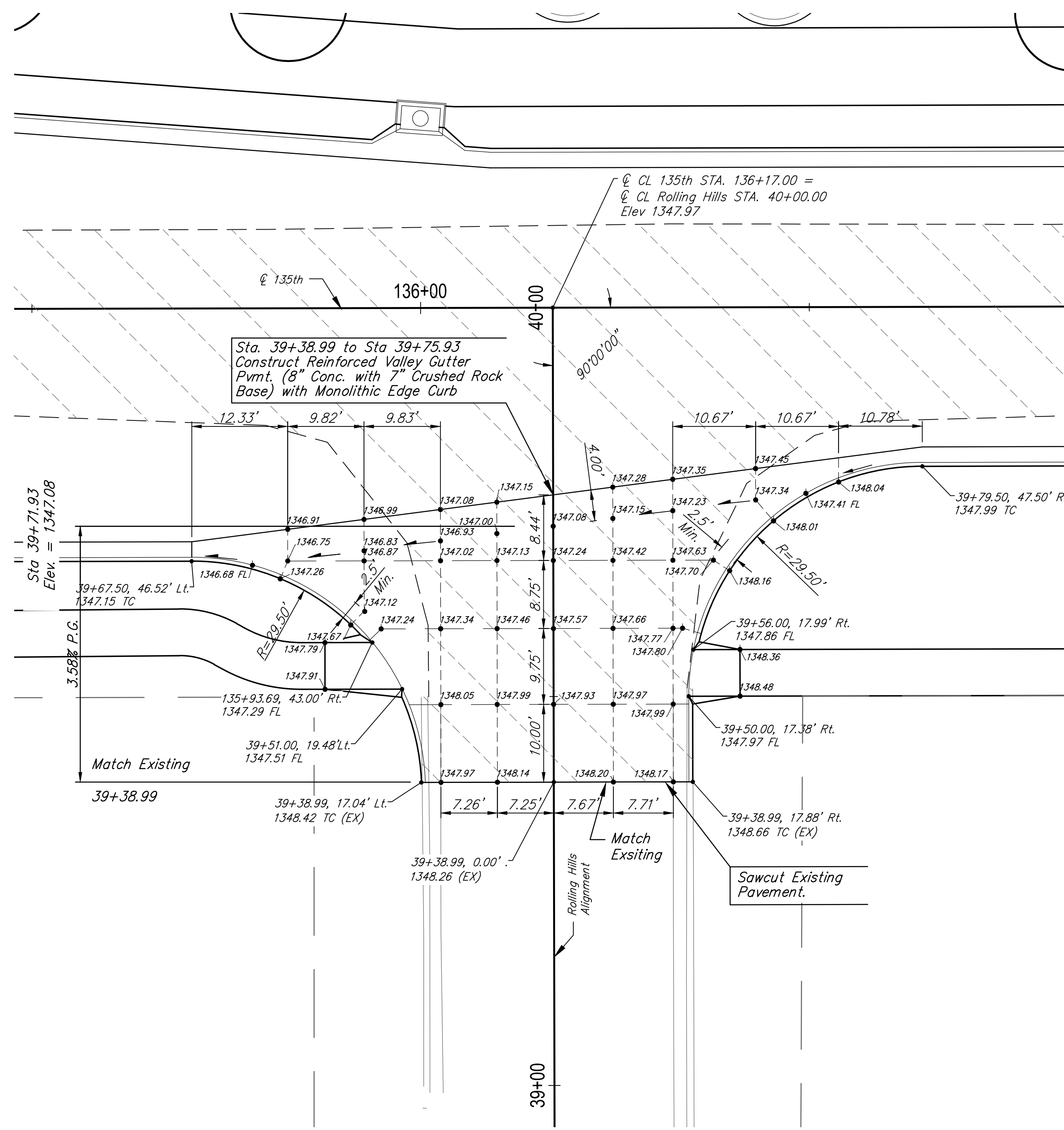
ROLLING HILLS STREET, STA 136+17
