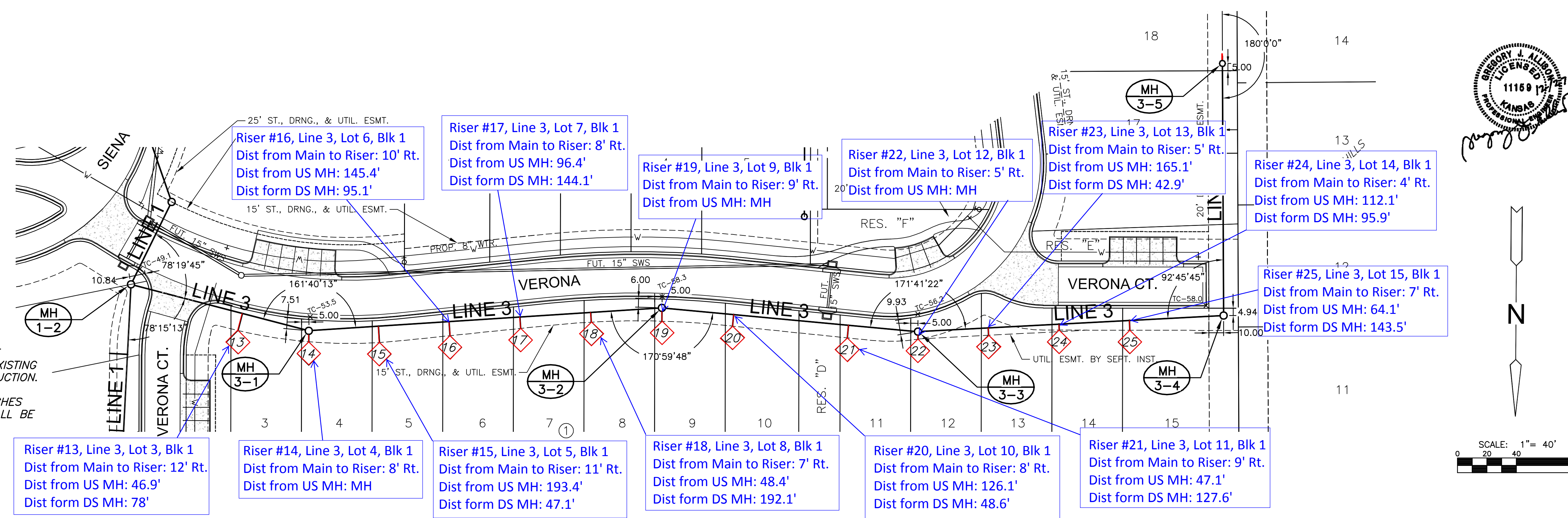
PLAN LINE 3 PROFILE LINE 3
