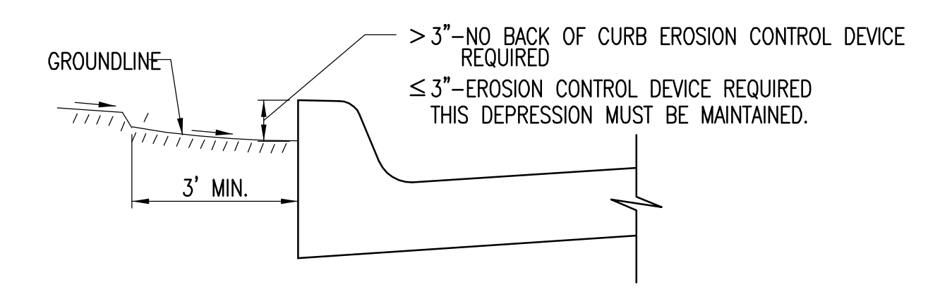
CURB BACKFILL DETAIL
