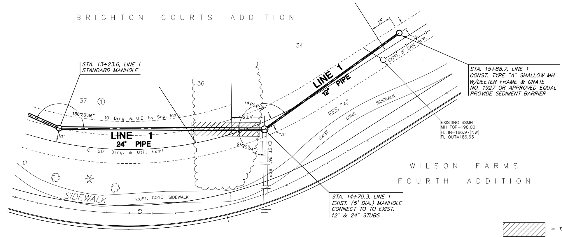
PLAN LINE 1
