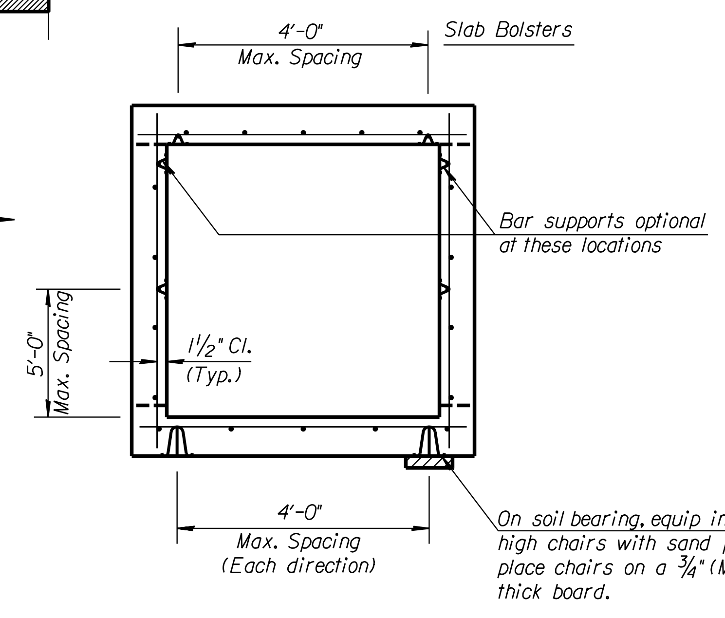
BOX CULVERT
