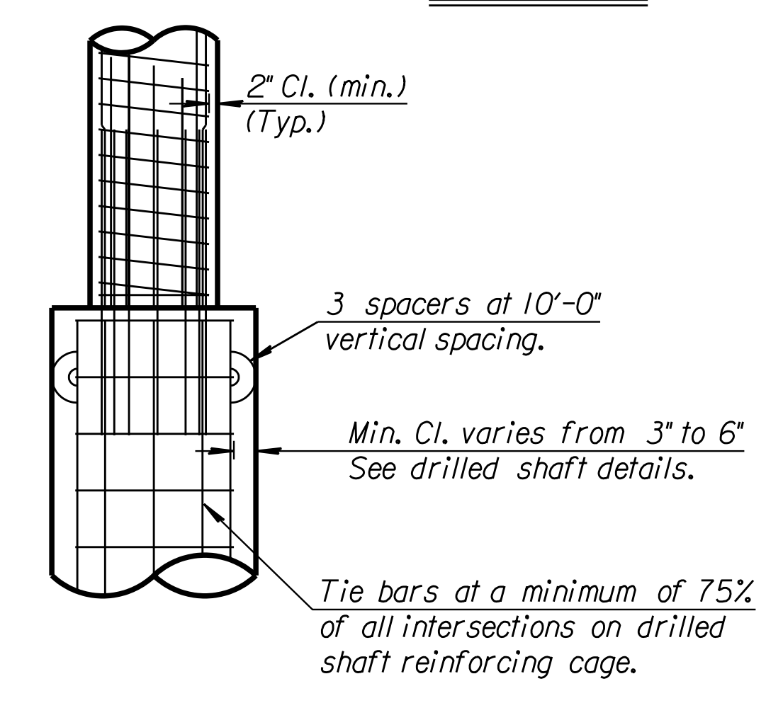
DRILLED SHAFT
