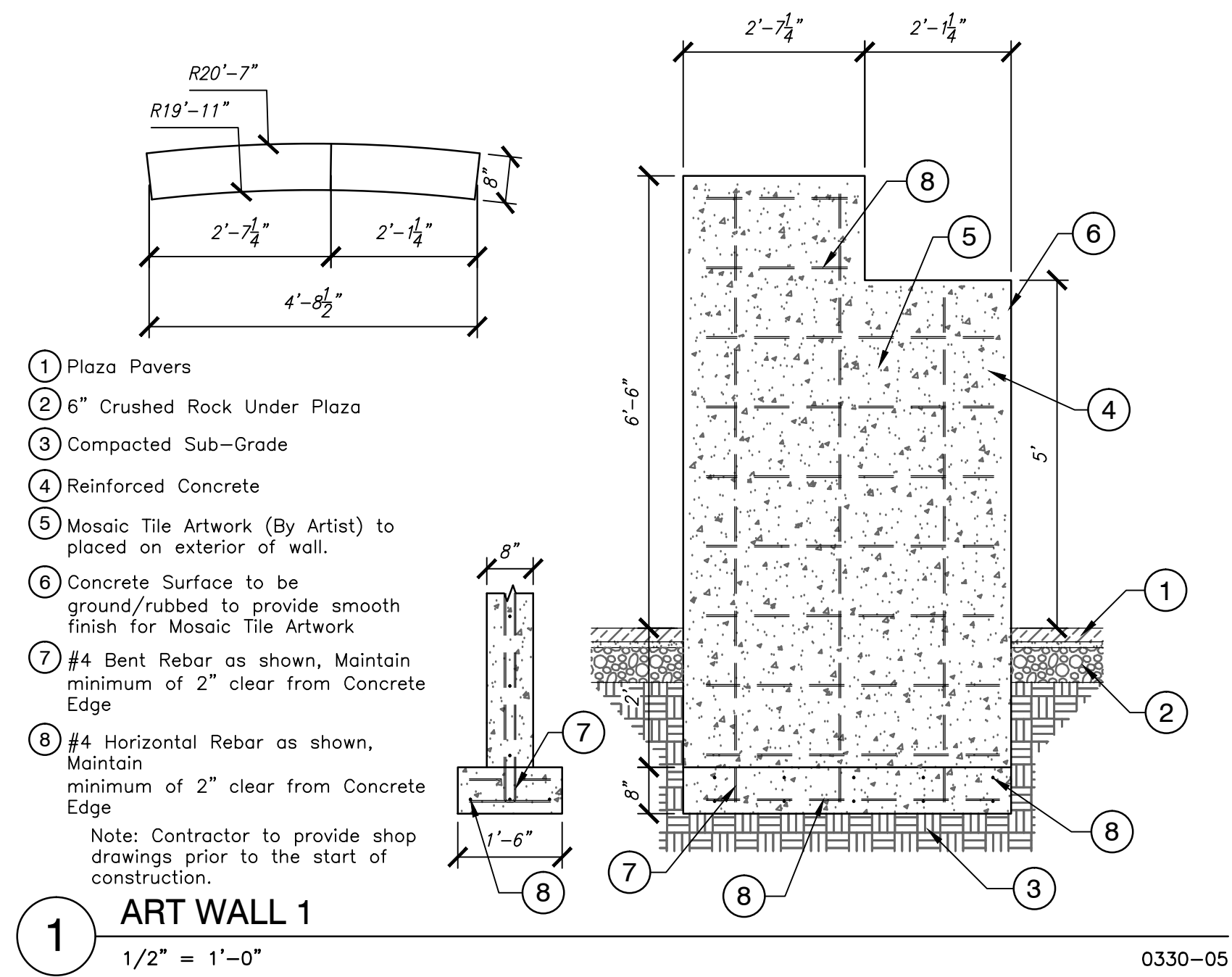
1 ART WALL 1 1/2" = 1'-0" 0330-05
