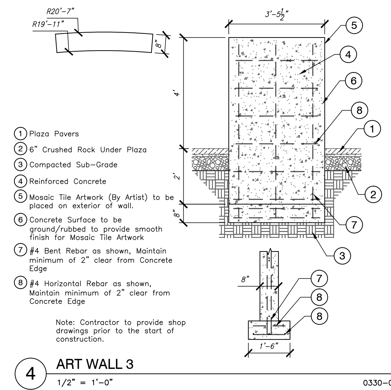
4 ART WALL 3 1/2" = 1'-0" 0330-08
