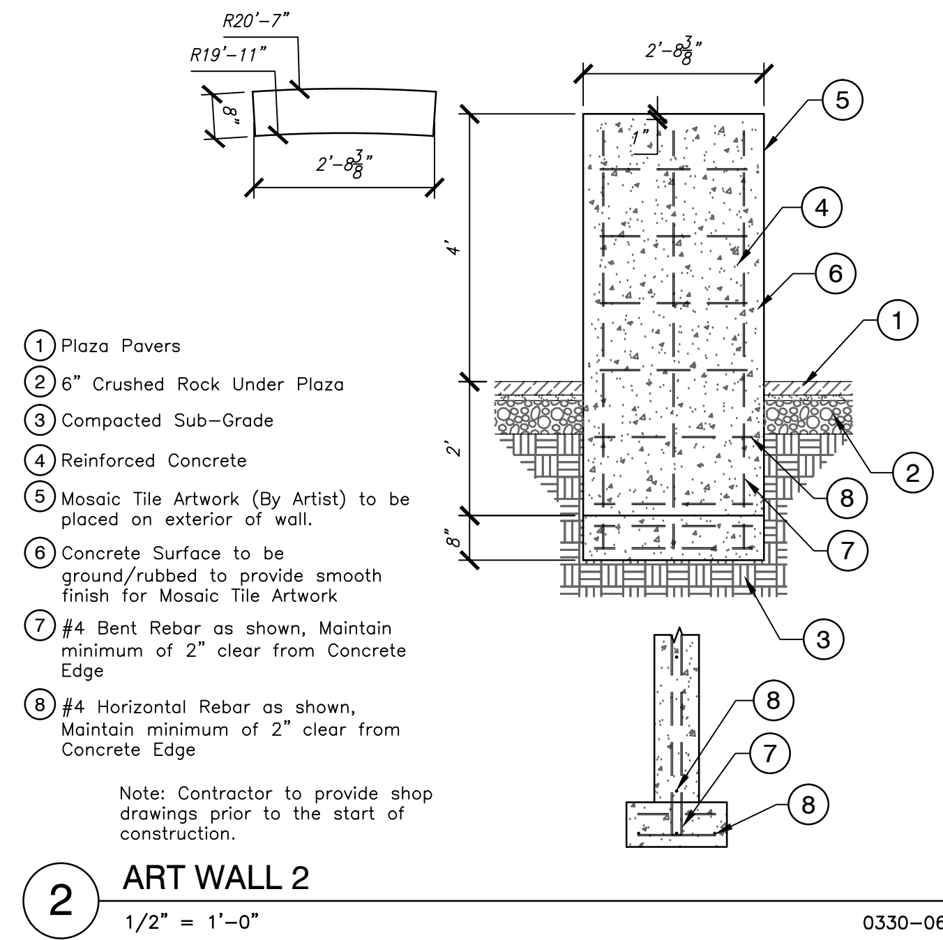
2 ART WALL 2 1/2" = 1'-0" 0330-06
