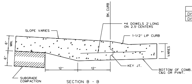
BACK OF CURB DETAIL
