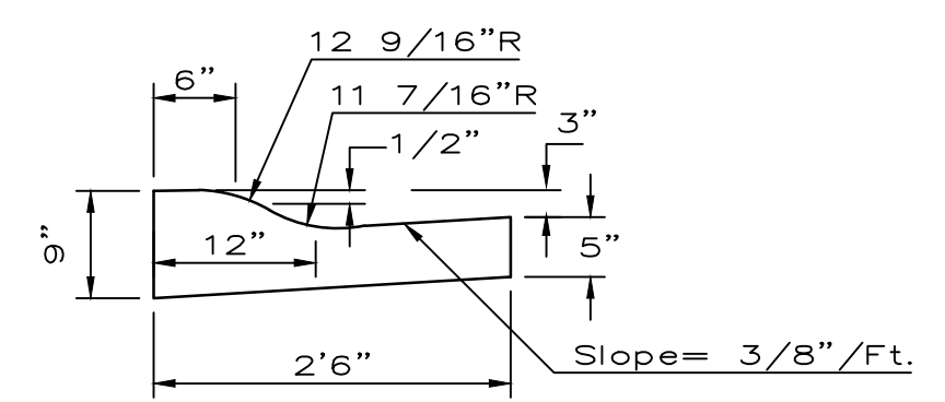
COMBINED ROLL TYPE CURB & GUTTER
