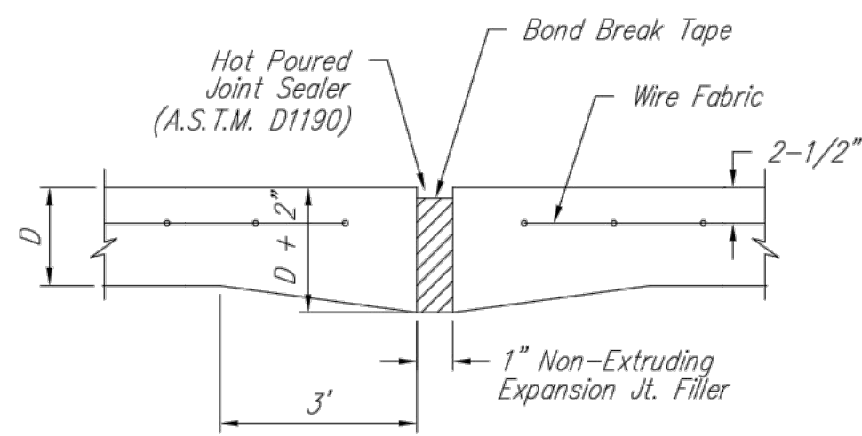
EXPANSION JOINT
