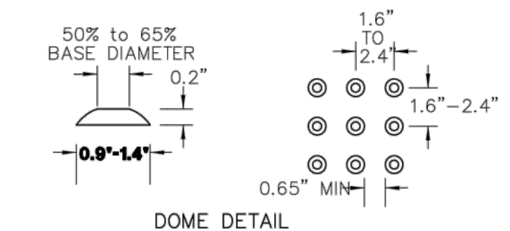
DOMES DETAIL
