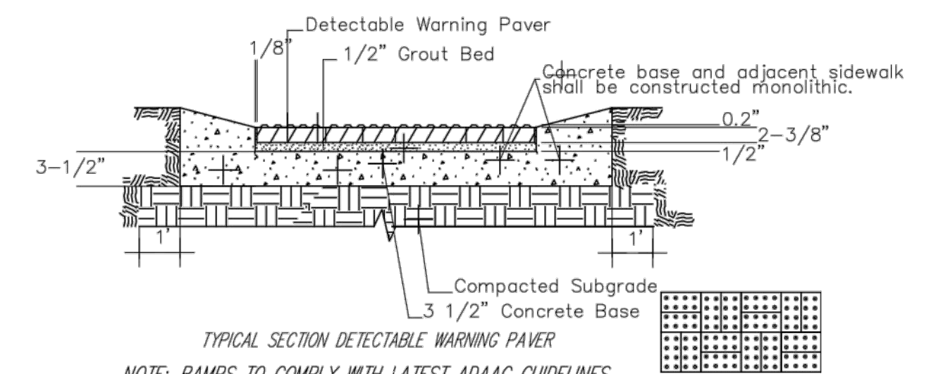
SECTION B-B
