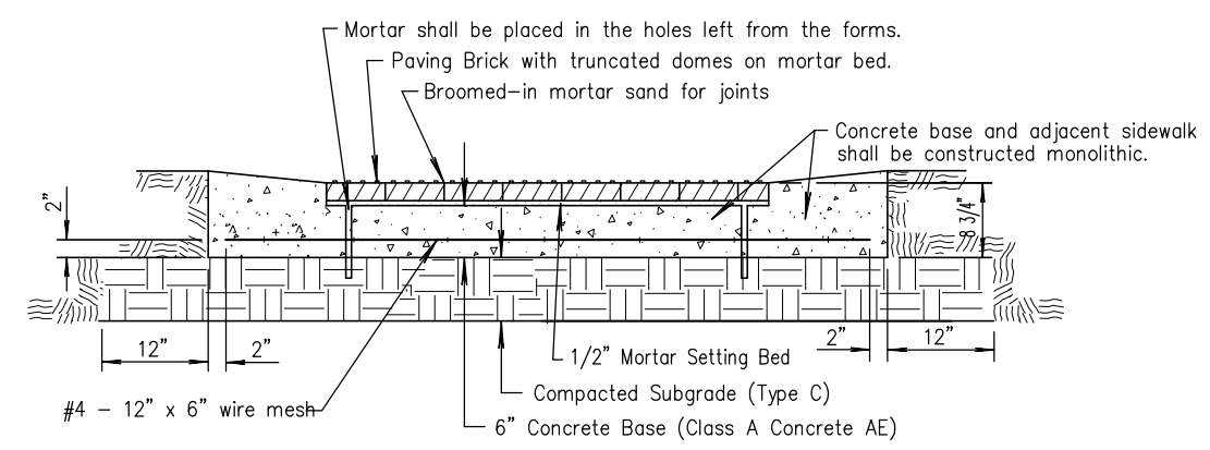
TYPICAL SECTION OF PAVER BRICK SECTION A-A
