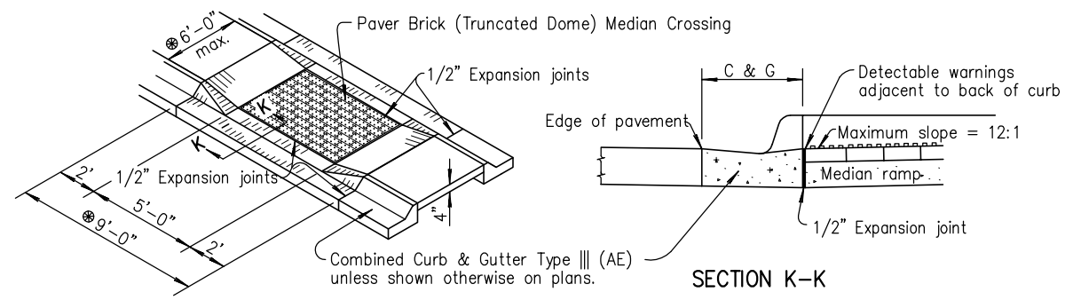
NARROW MEDIAN RAMP CROSSING
