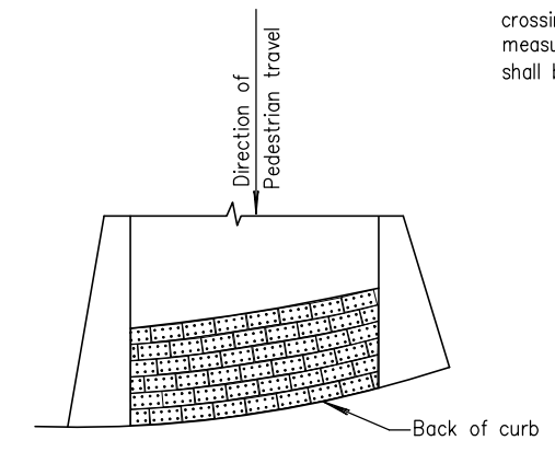
RADIUS CURB DETAILS
