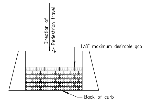
STRAIGHT CURB DETAILS
