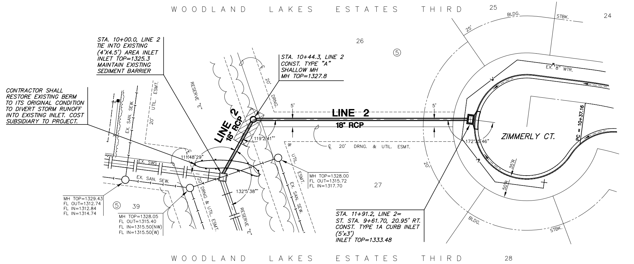
PLAN LINE 2 SCALE: 1"=20' ▨ = PROTECTIVE FILL ▨ = TREE REMOVAL
