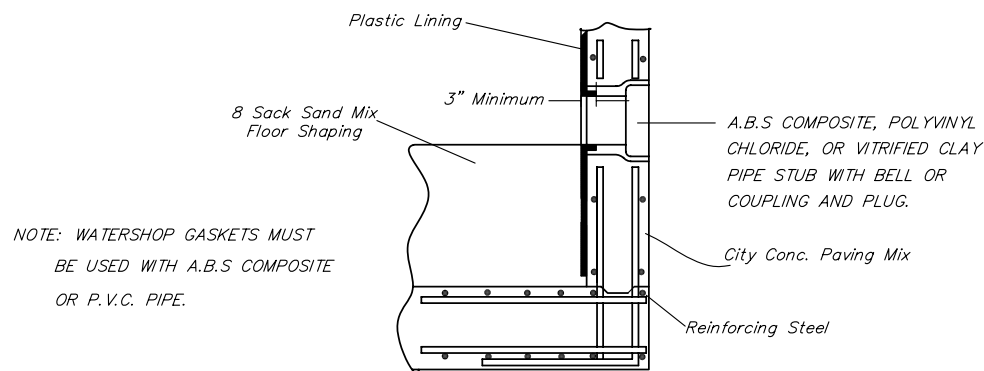
PIPE STUB DETAIL SANITARY SEWER ONLY
