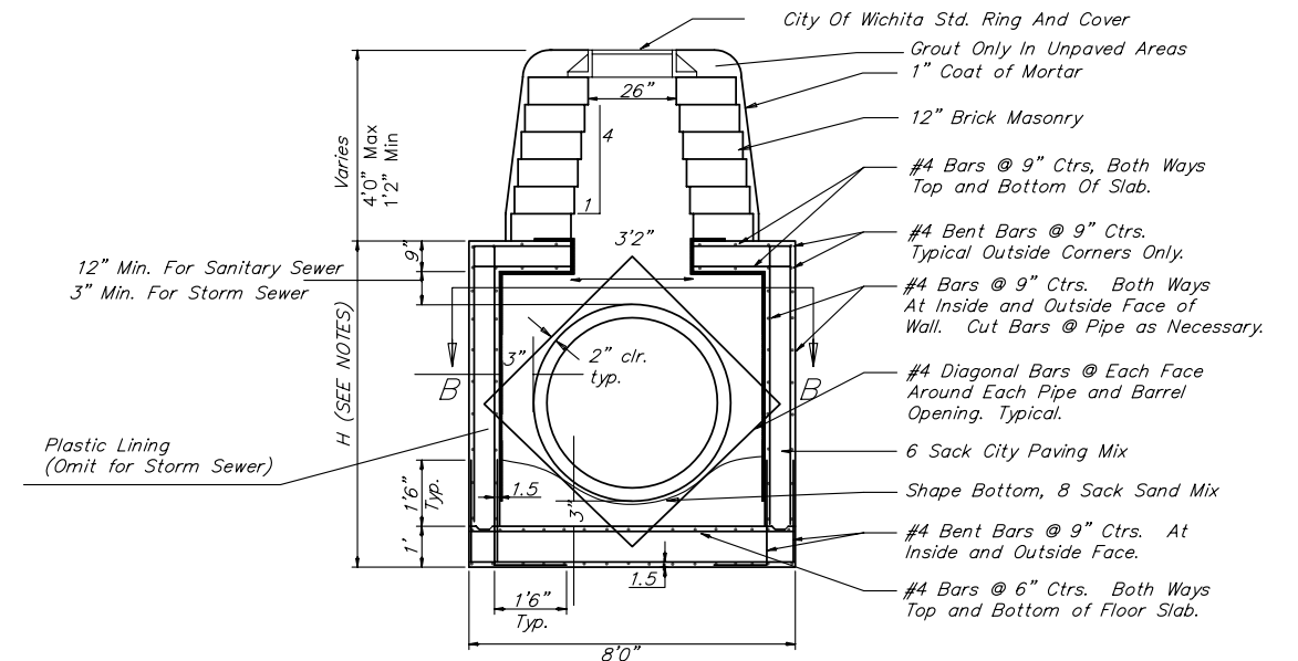
REINFORCED CONCRETE MANHOLE MANHOLE STACK 2.33' TO 4'0"
