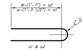
BENDING DIAGRAM
