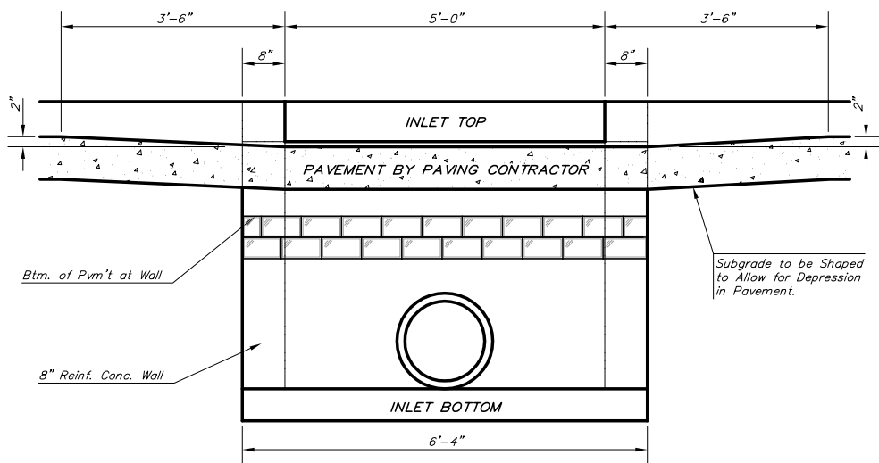
SECTION E-E
