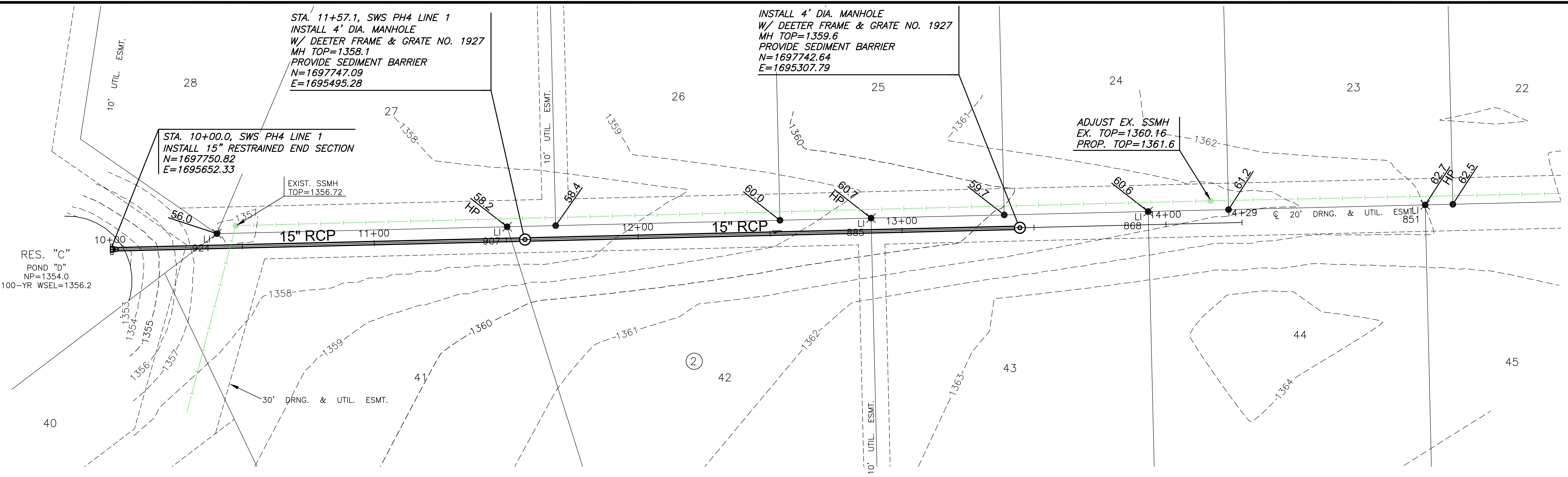
PLAN SWS PHASE 4 LINE 1 PROFILE SWS PHASE 4 LINE 1
