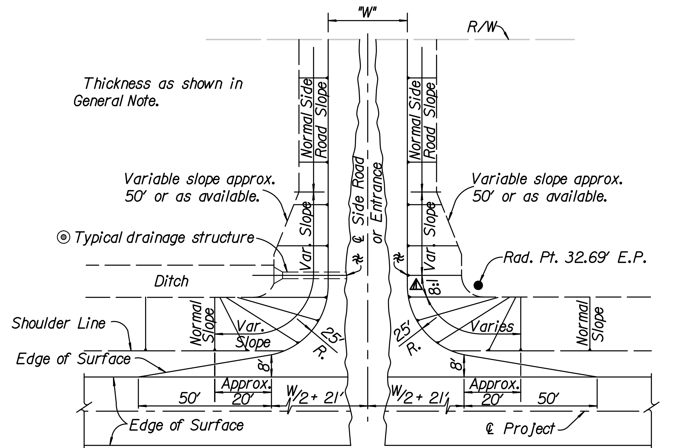
WITH DRAINAGE STRUCTURE MOUND ENTRANCE OR SIDE ROAD DETAIL FOR SURFACING OF SIDE ROADS & HOUSE ENTRANCES
