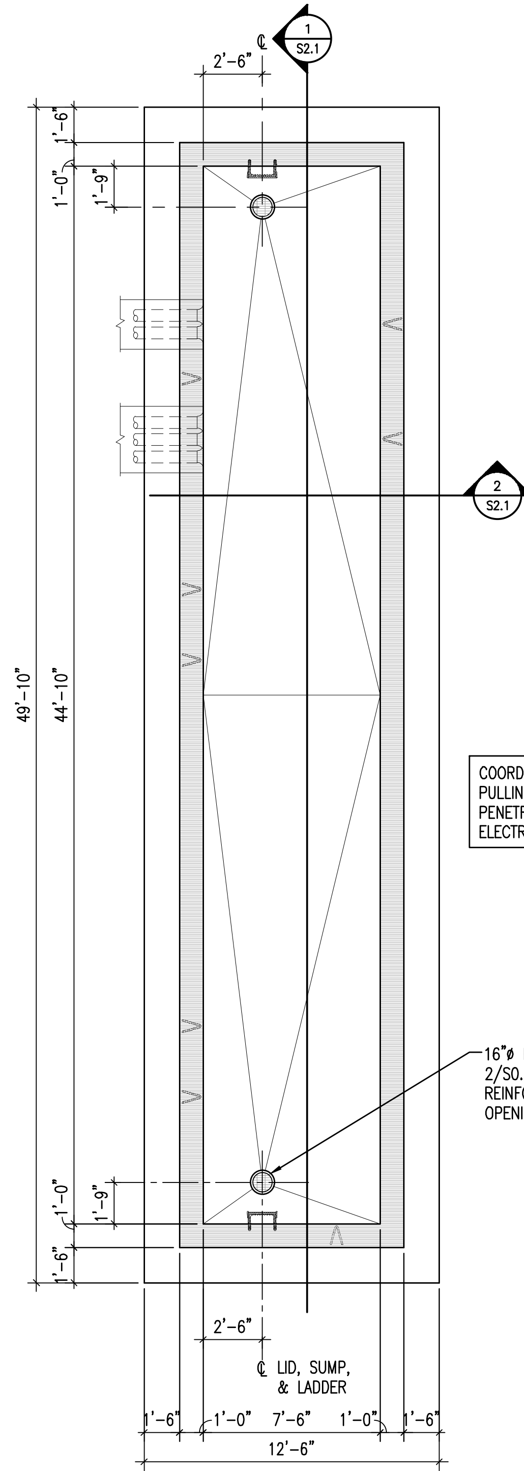
2 VAULT FOUNDATION PLAN S1.1 1/4"=1'0"
