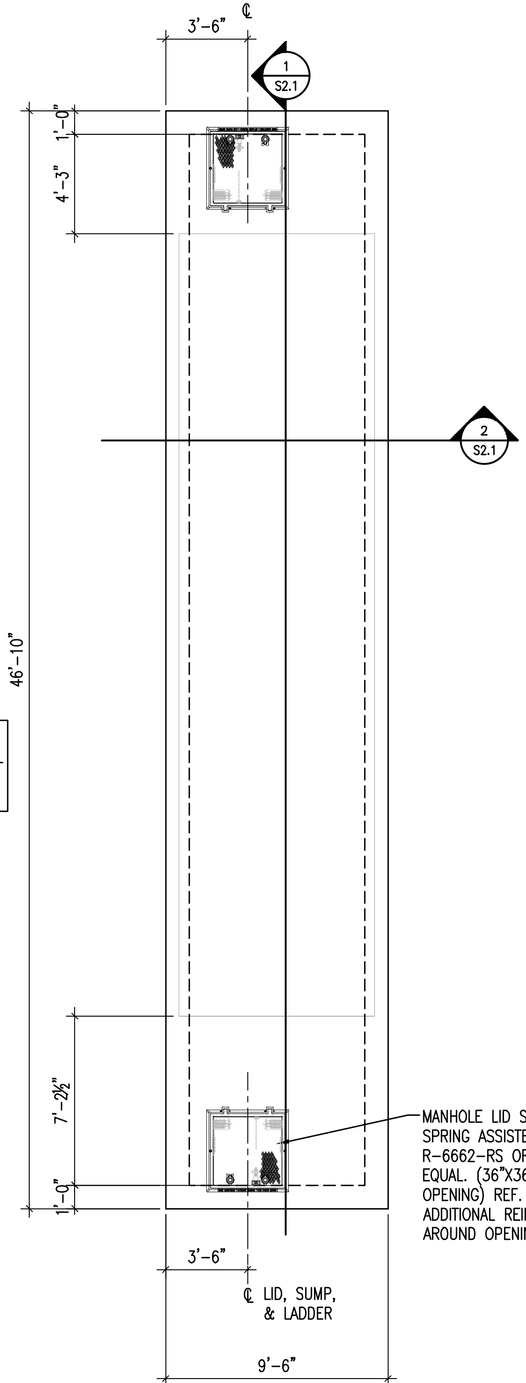
3 VAULT COVER PLAN S1.1 1/4"=1'0"
