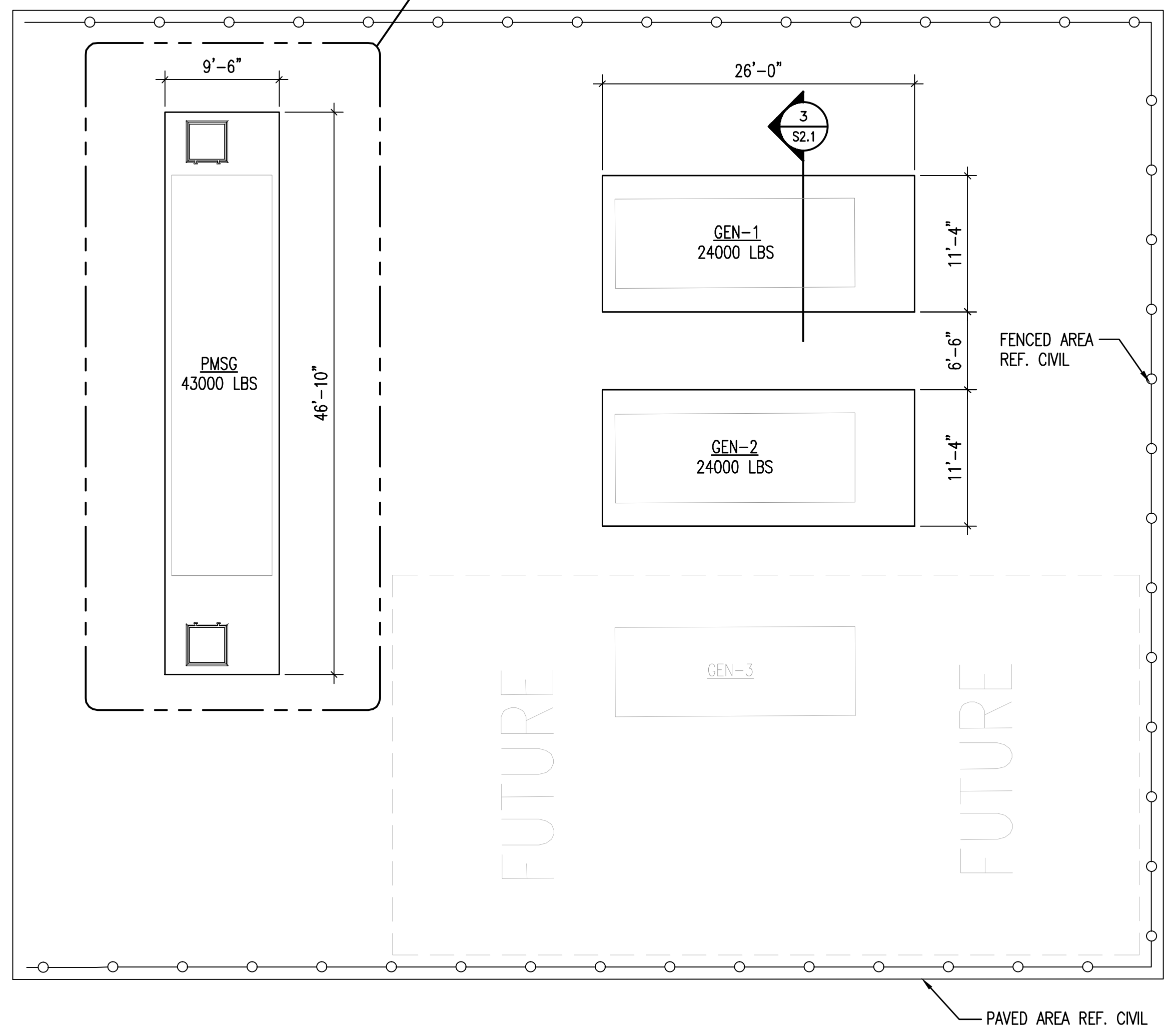
1 EQUIPMENT PLAN S1.1 1/8"=1'0"
