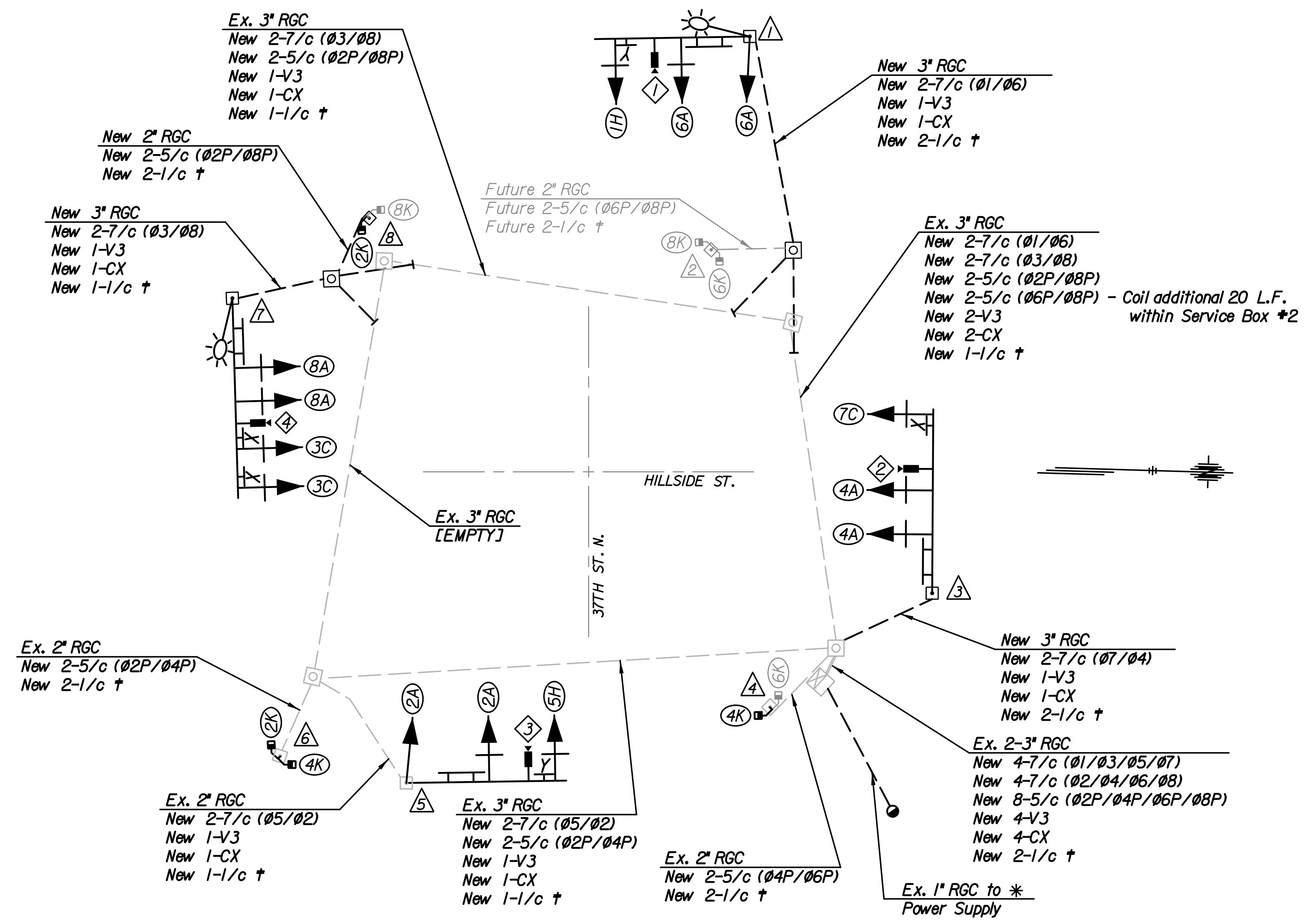
WIRING DIAGRAM NOT TO SCALE
