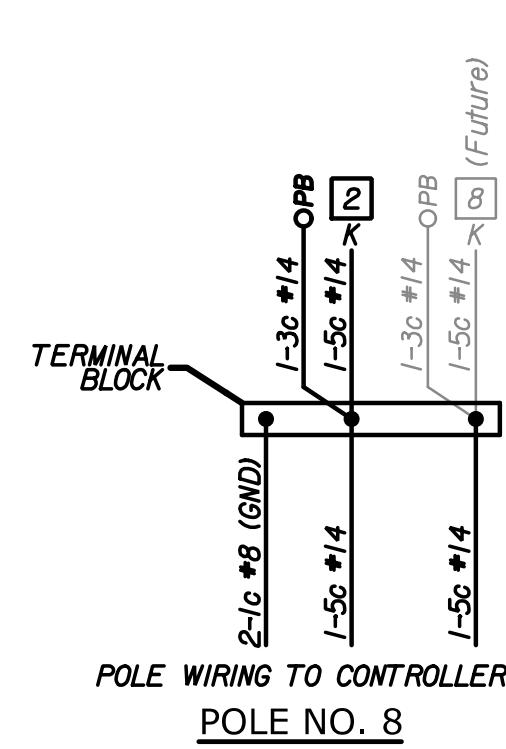
POLE WIRING DIAGRAM NOT TO SCALE
