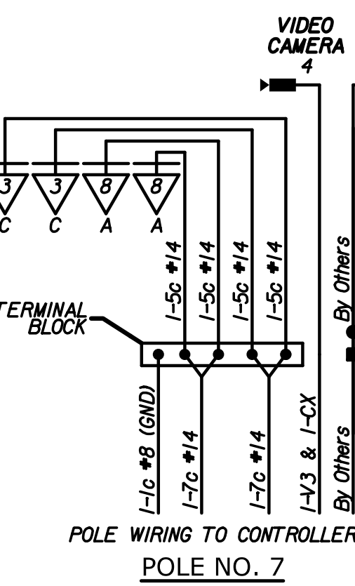
POLE WIRING DIAGRAM NOT TO SCALE
