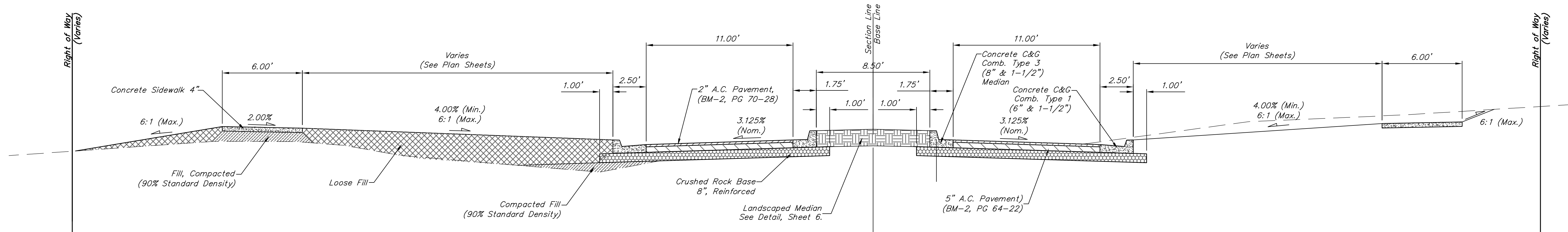
TYLER ROAD TYPICAL SECTION Sta. 20+25.00 to Sta. 22+00.00
